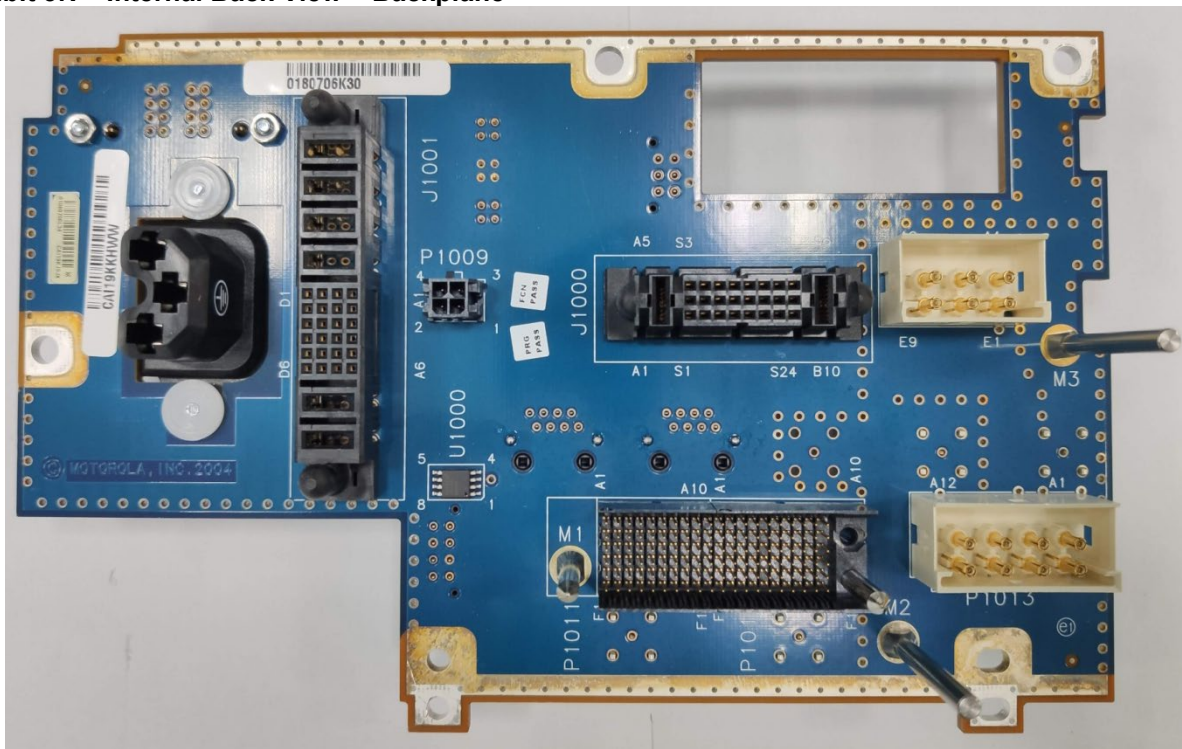
Exhibit 3N – Internal Back View – Backplane
