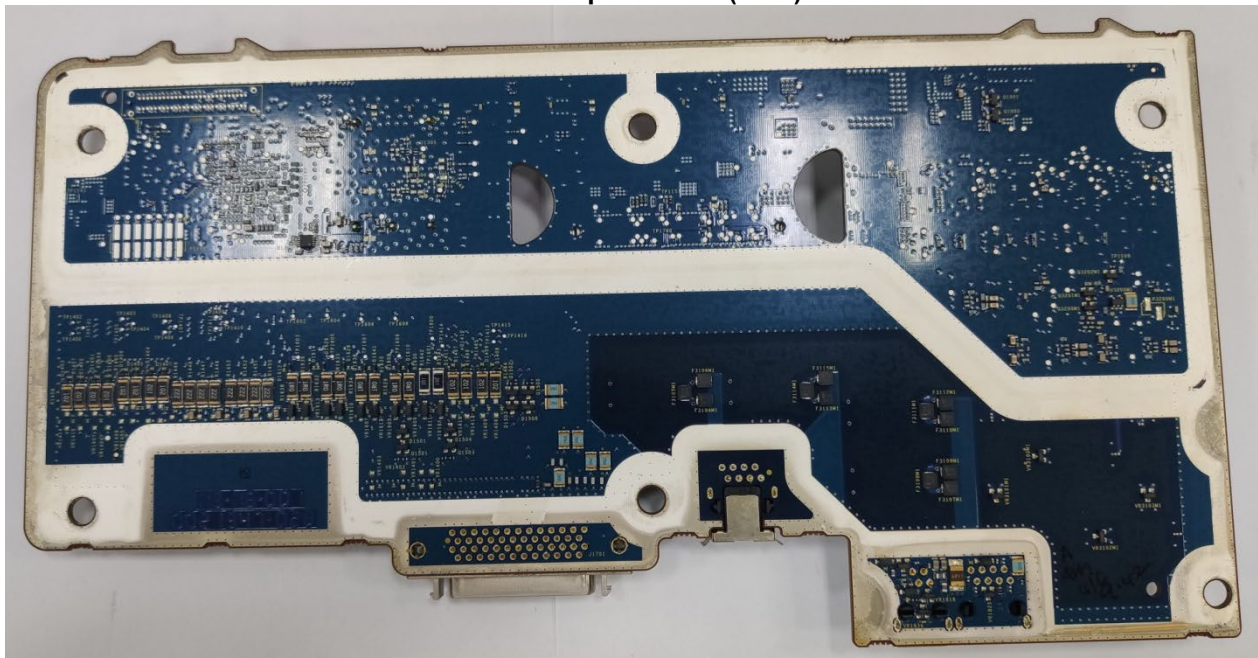
Exhibit 3O – Internal Back View – Transceiver Option Card (TOC)
