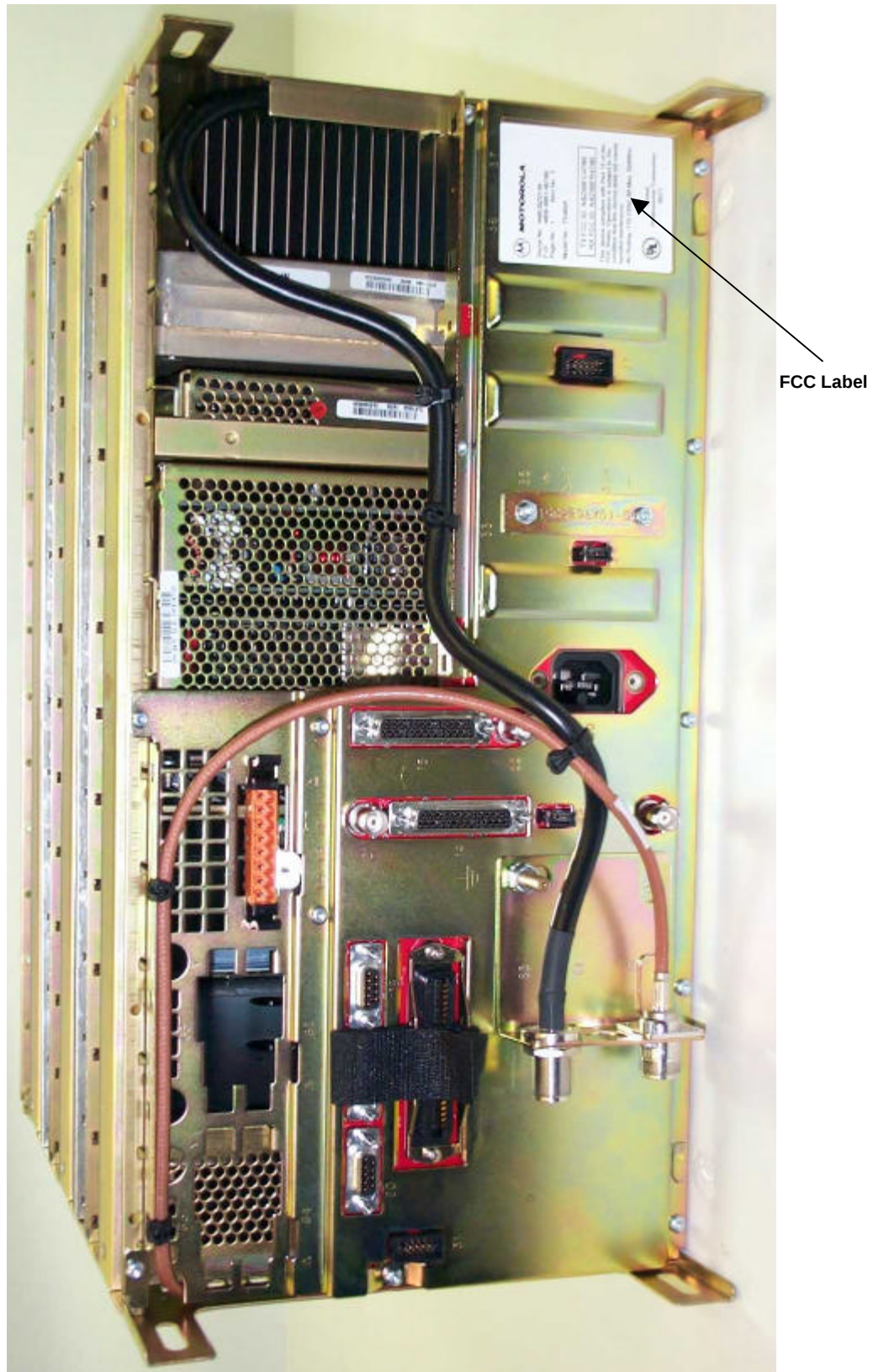
Rear of Base Radio Including Location of the FCC ID Label
