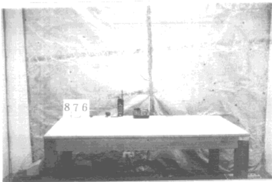
Fig. 2 Conducted Emissions Test Configuration (Operating only)
