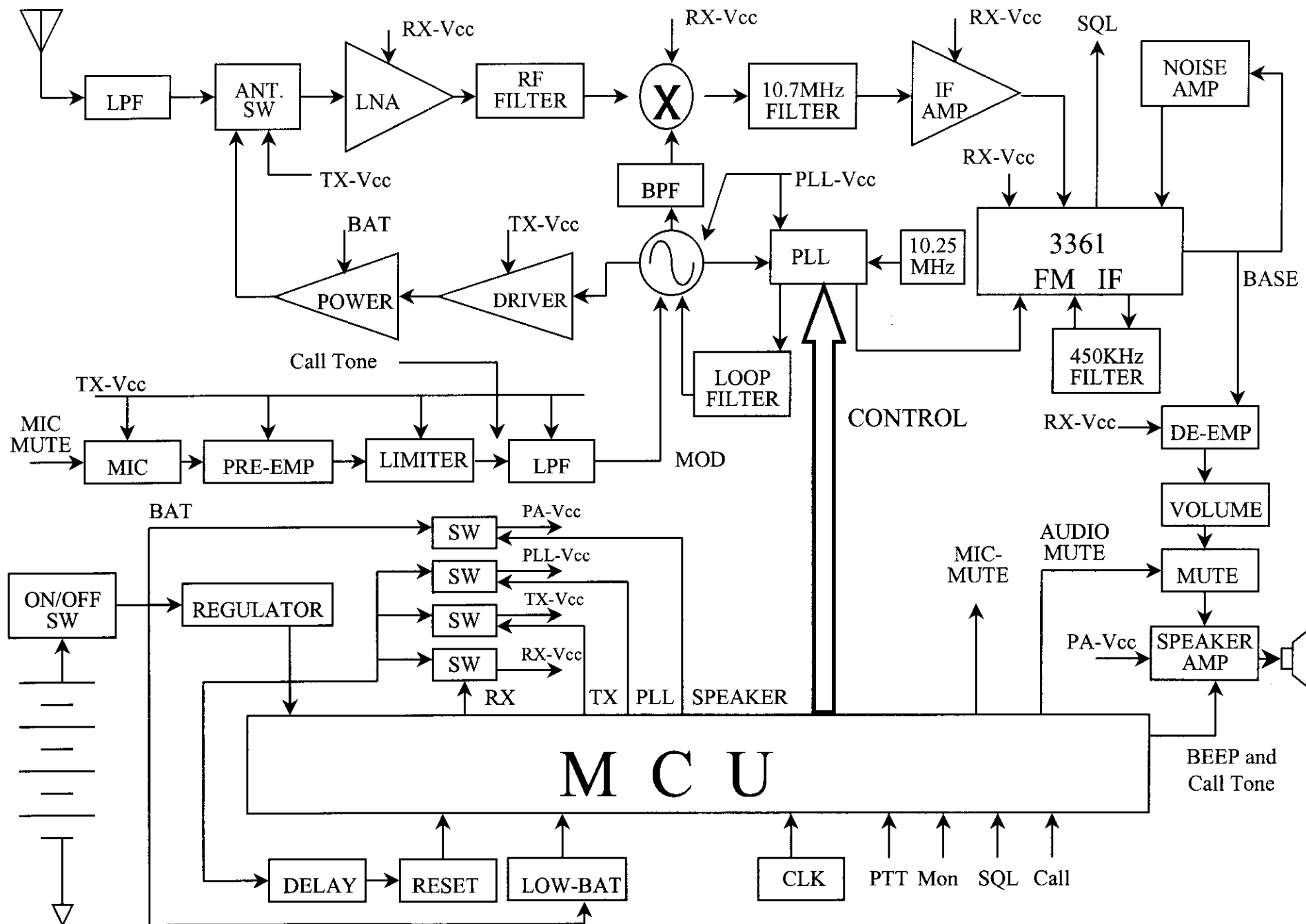
21-1855 14-channel FRS radio block diagram
