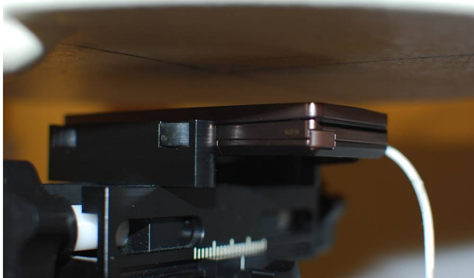
Figure 19-10 SAR Test Setup Photo 10
