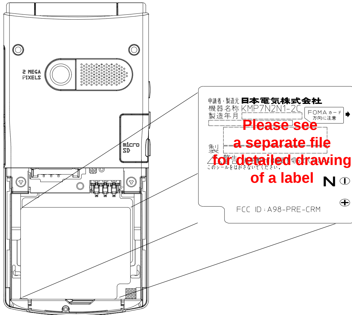
Rear View Without Battery Pack
