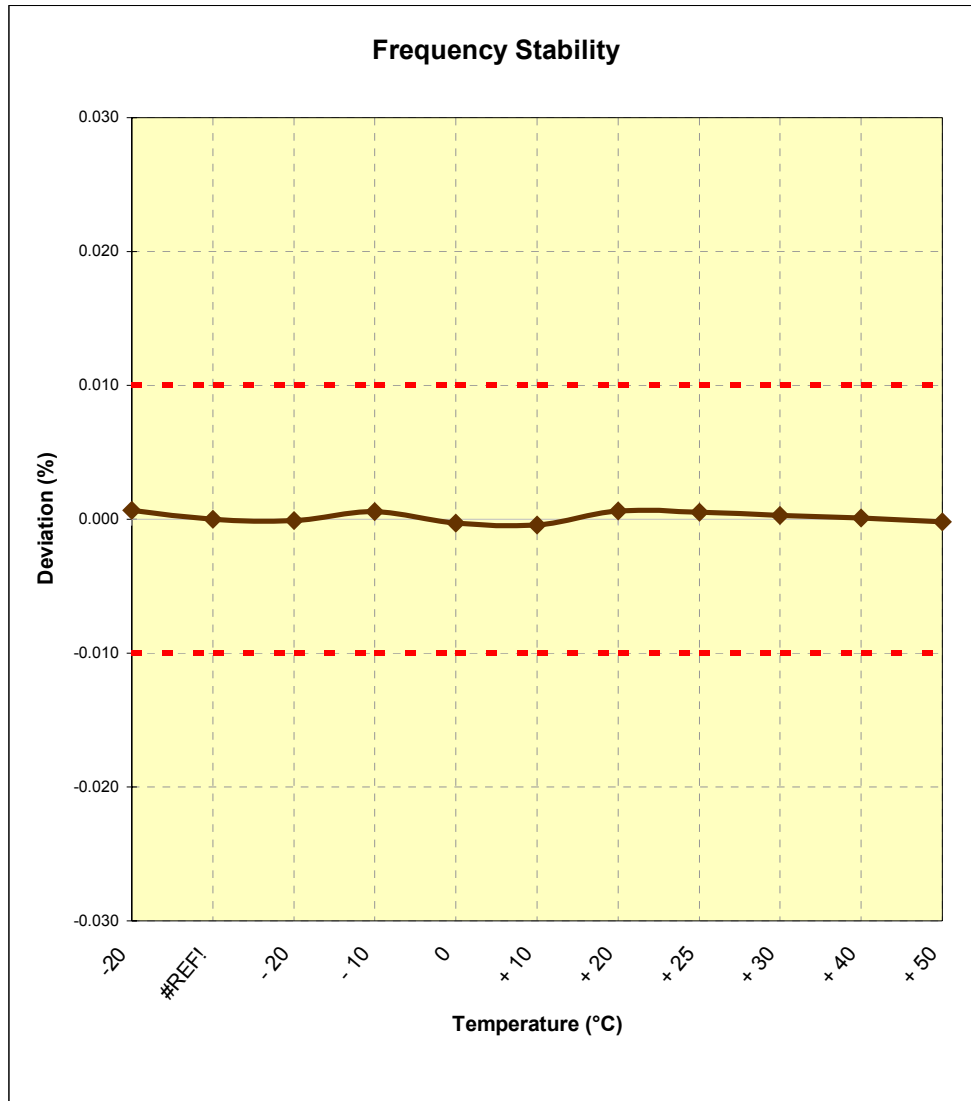
Figure 8-3. Frequency Stability Plot
