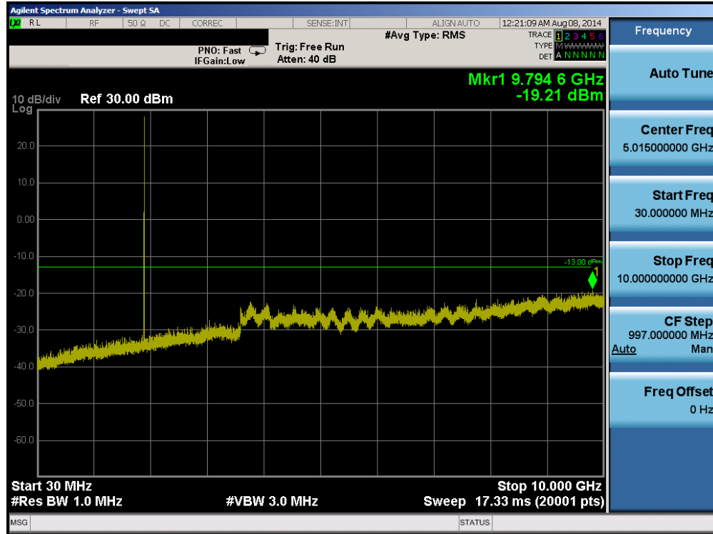
Plot 6-7. Conducted Spurious Plot (PCS GSM Mode – Ch. 810)
