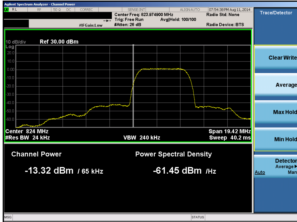
Plot 6-17. Band Edge Plot (Cellular WCDMA Mode – Ch. 4132)
