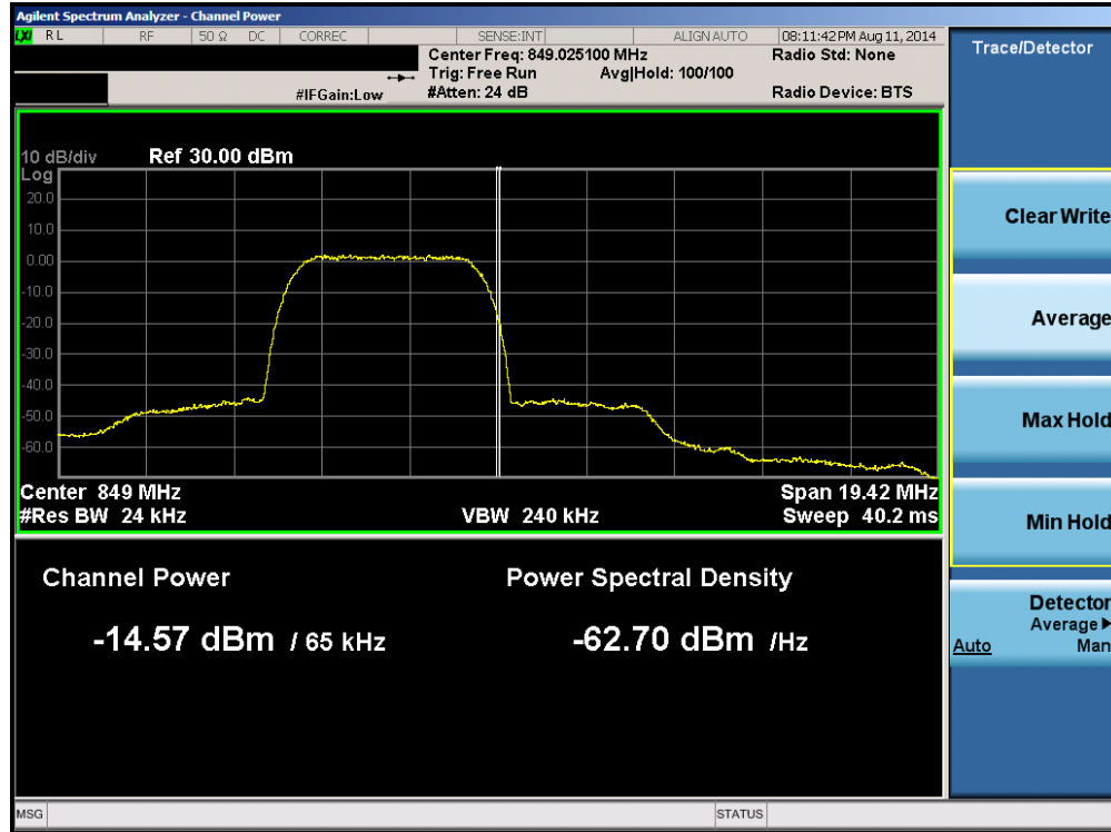
Plot 6-19. Band Edge Plot (Cellular WCDMA Mode – Ch. 4233)
