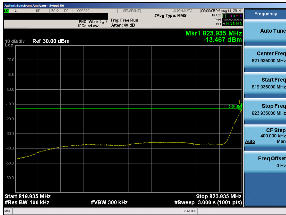
Plot 6-18. 4MHz Span Plot (Cellular WCDMA Mode – Ch. 4132)
