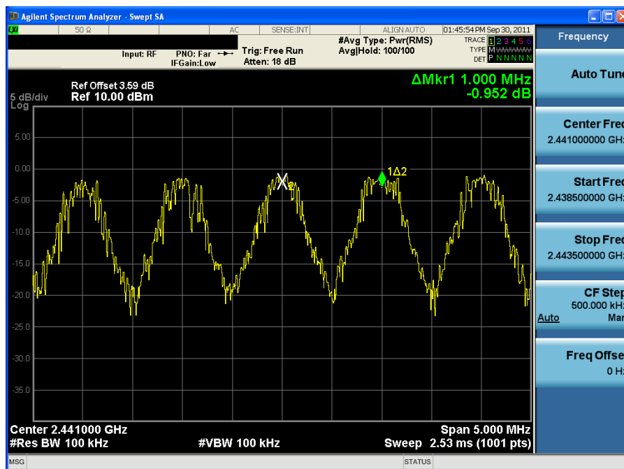
Plot 6-15. Channel Spacing Plot (Bluetooth)
