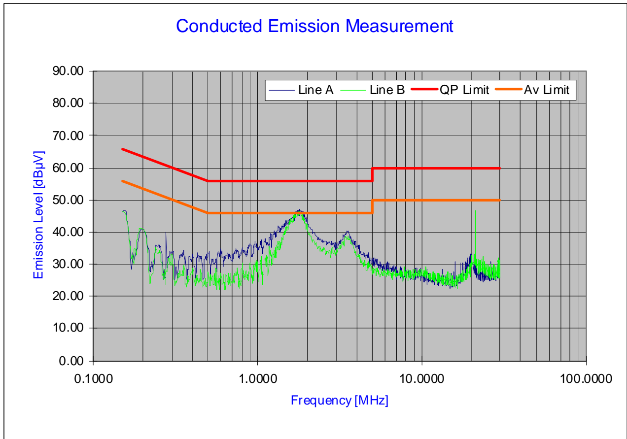
Plot 6-37. Line Conducted Plot with 802.11n
