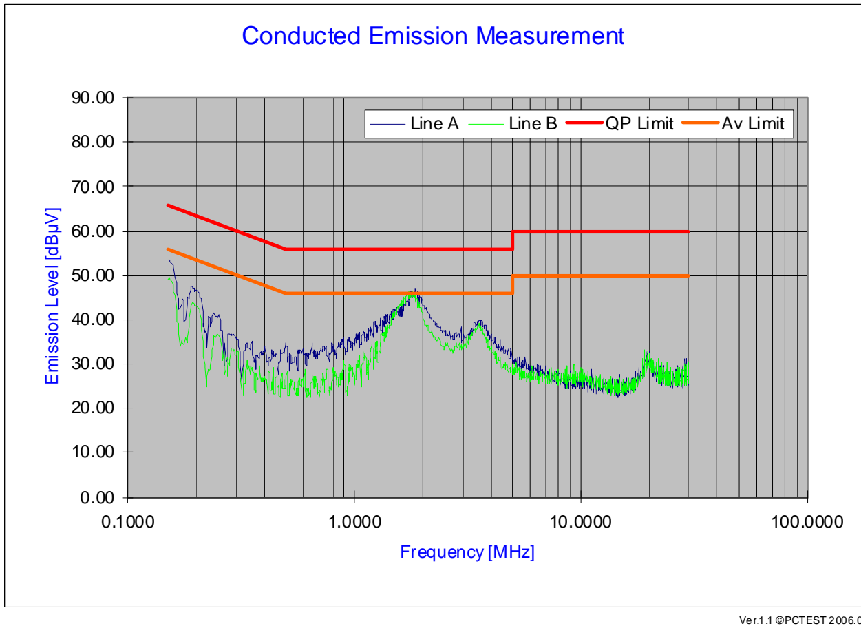
Plot 6-35. Line Conducted Plot with 802.11b
