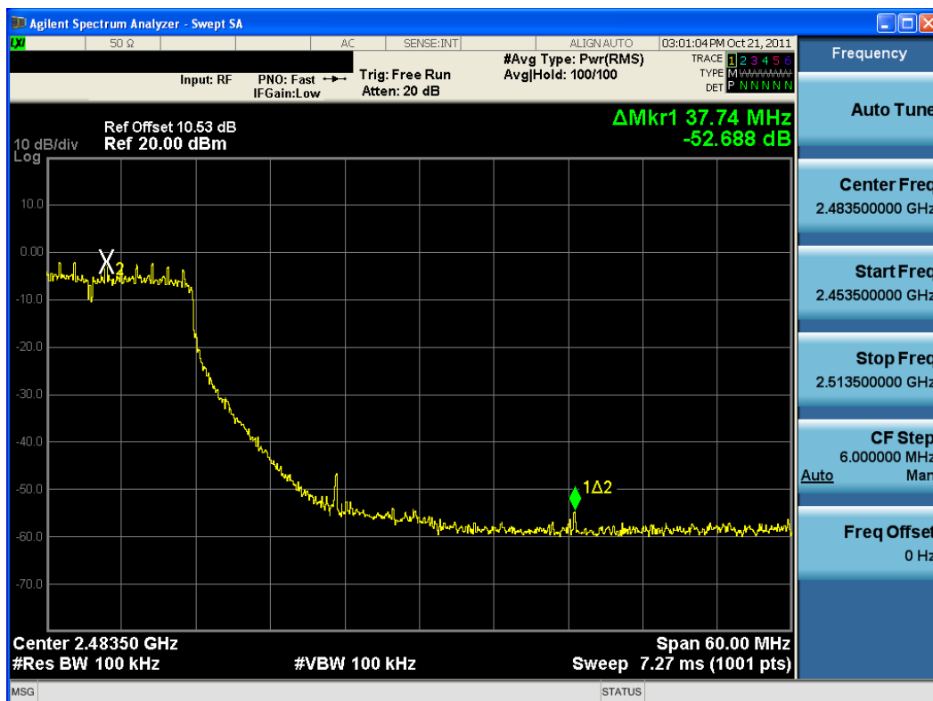
Plot 6-23. Band Edge Plot (802.11g – Ch. 10)
