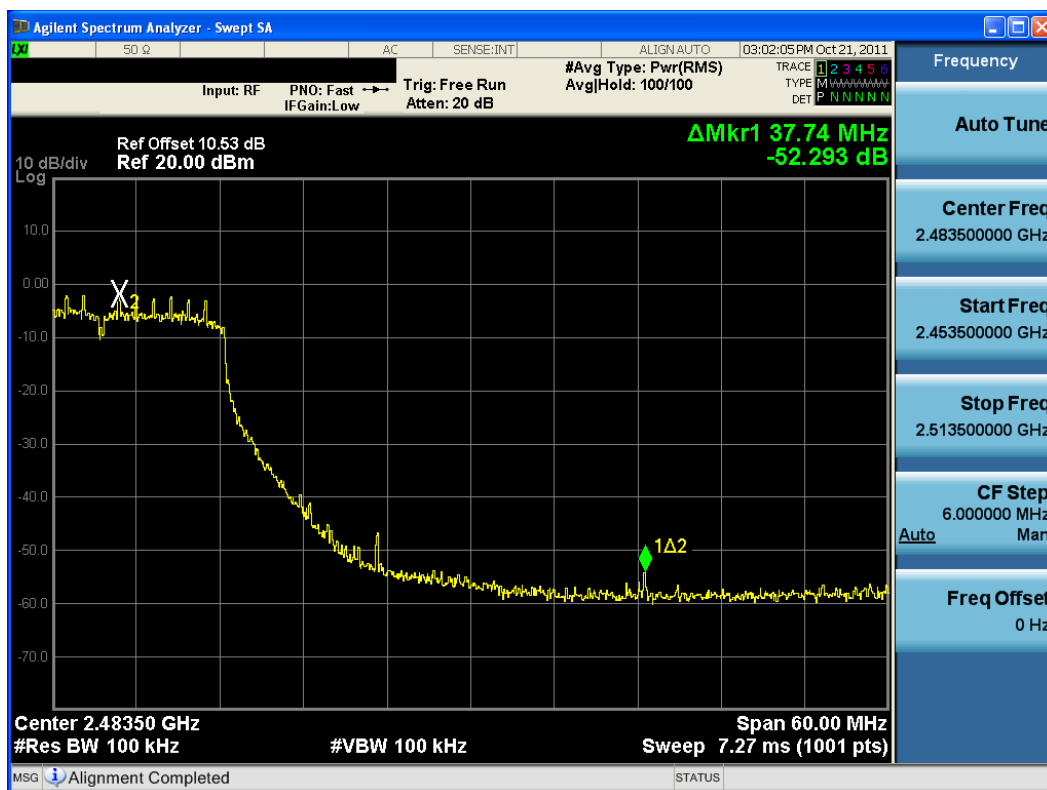
Plot 6-27. Band Edge Plot (802.11n – Ch. 10)
