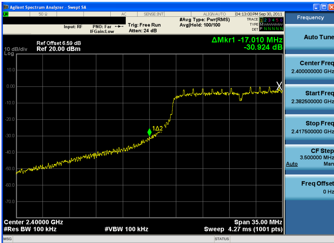
Plot 6-25. Band Edge Plot (802.11n – Ch. 1)
