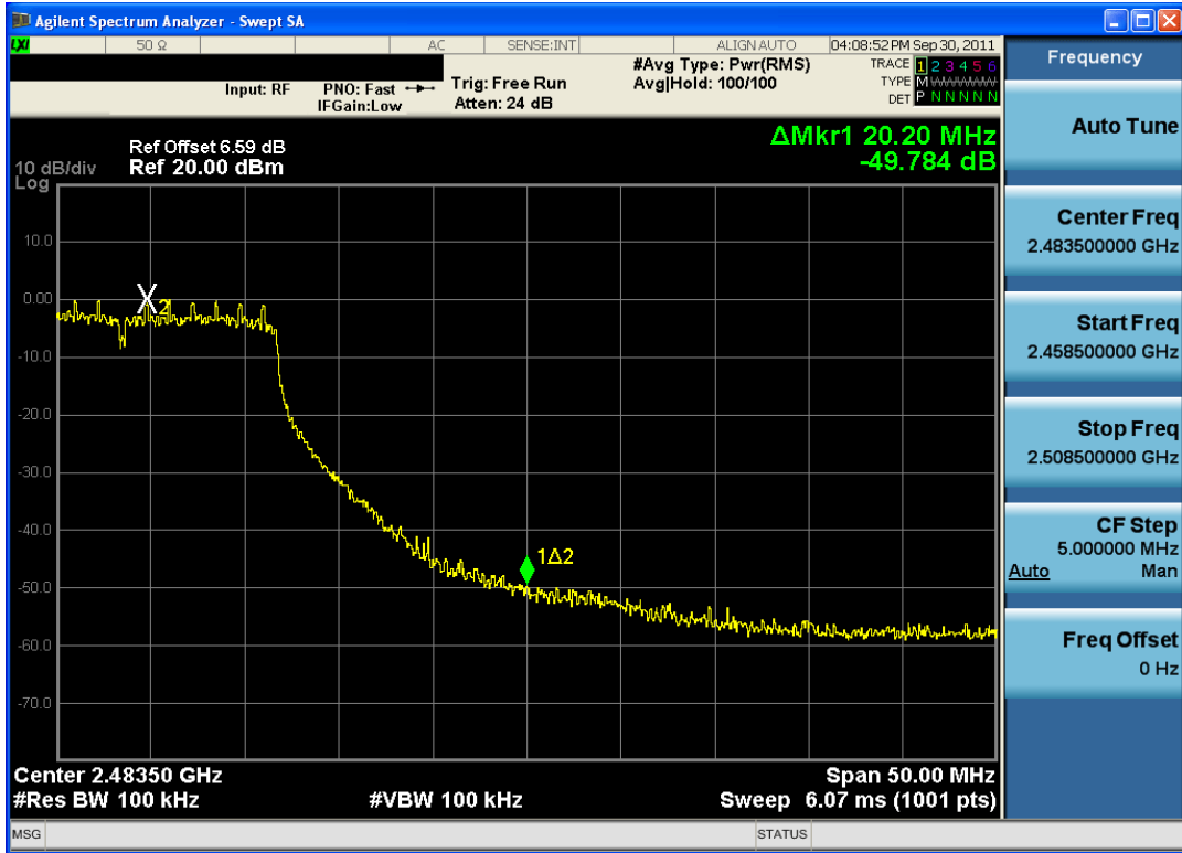
Plot 6-24. Band Edge Plot (802.11g – Ch. 11)
