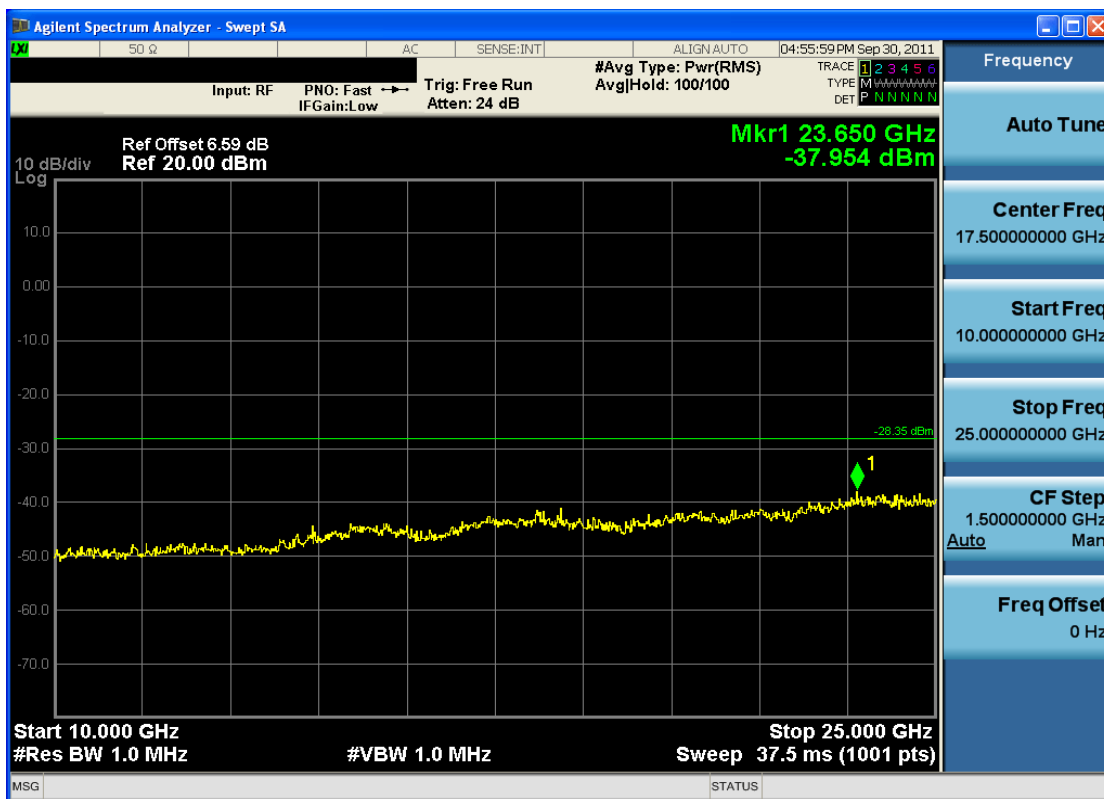
Plot 6-30. Conducted Spurious Plot (802.11b – Ch. 1)
