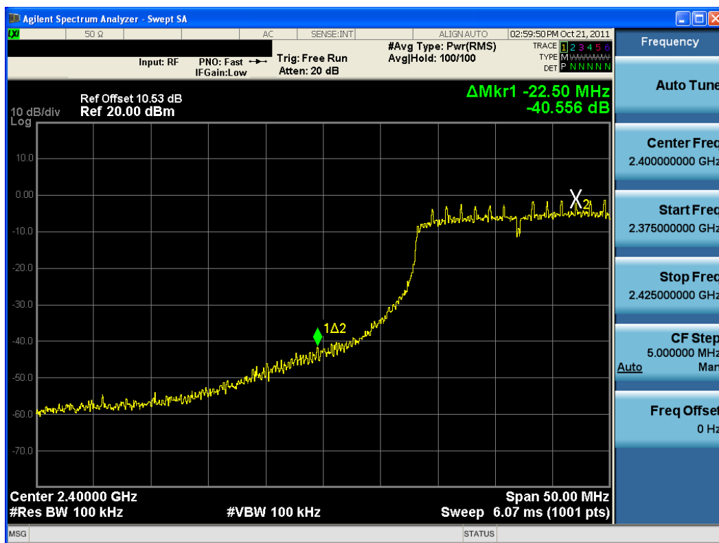
Plot 6-26. Band Edge Plot (802.11n – Ch. 2)
