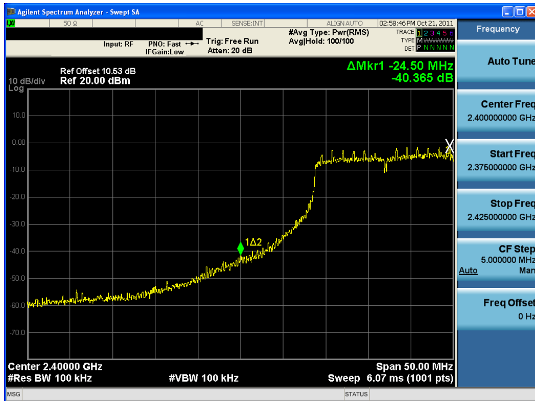
Plot 6-22. Band Edge Plot (802.11g – Ch. 2)
