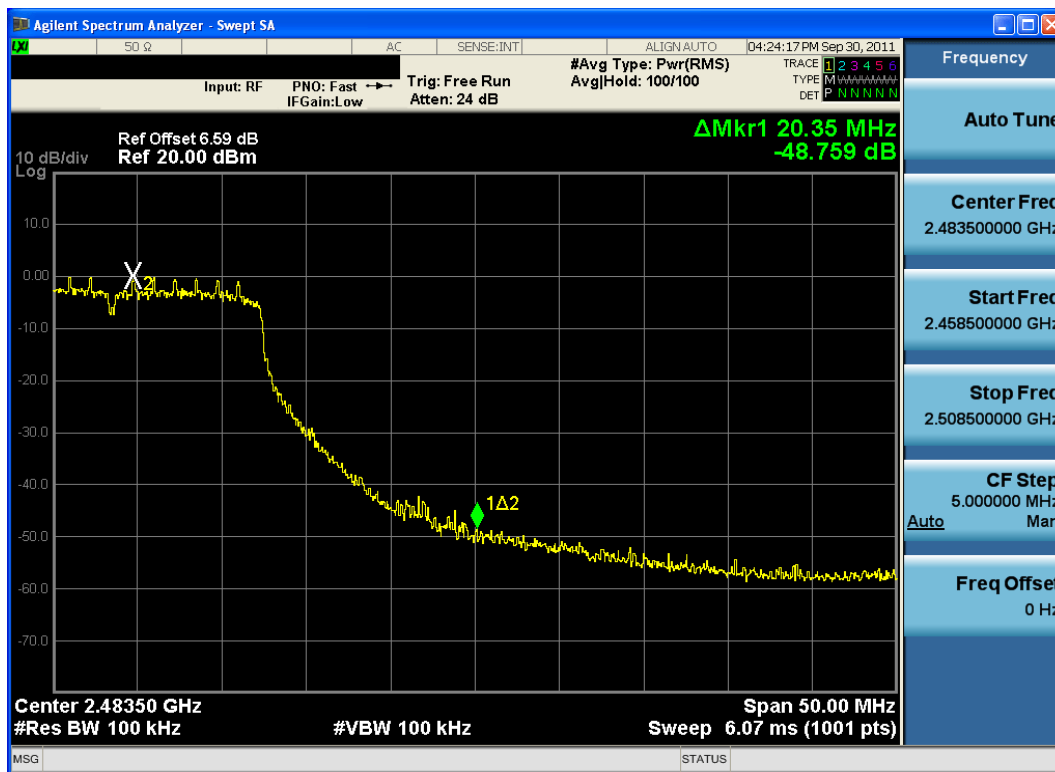
Plot 6-28. Band Edge Plot (802.11n – Ch. 11)
