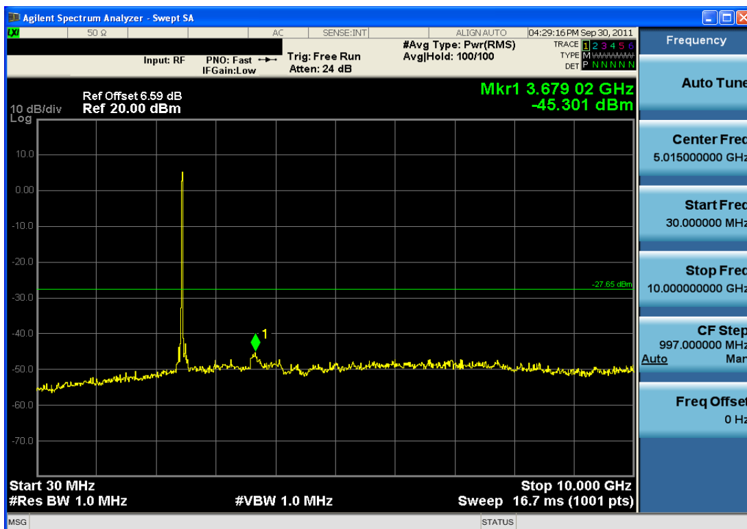
Plot 6-33. Conducted Spurious Plot (802.11b – Ch. 11)
