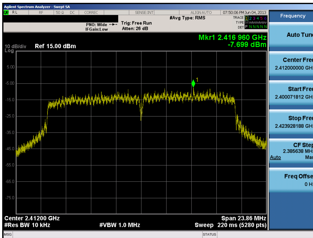
Plot 6-22. Power Spectral Density Plot (802.11n SGI (2.4GHz) – Ch. 1)
