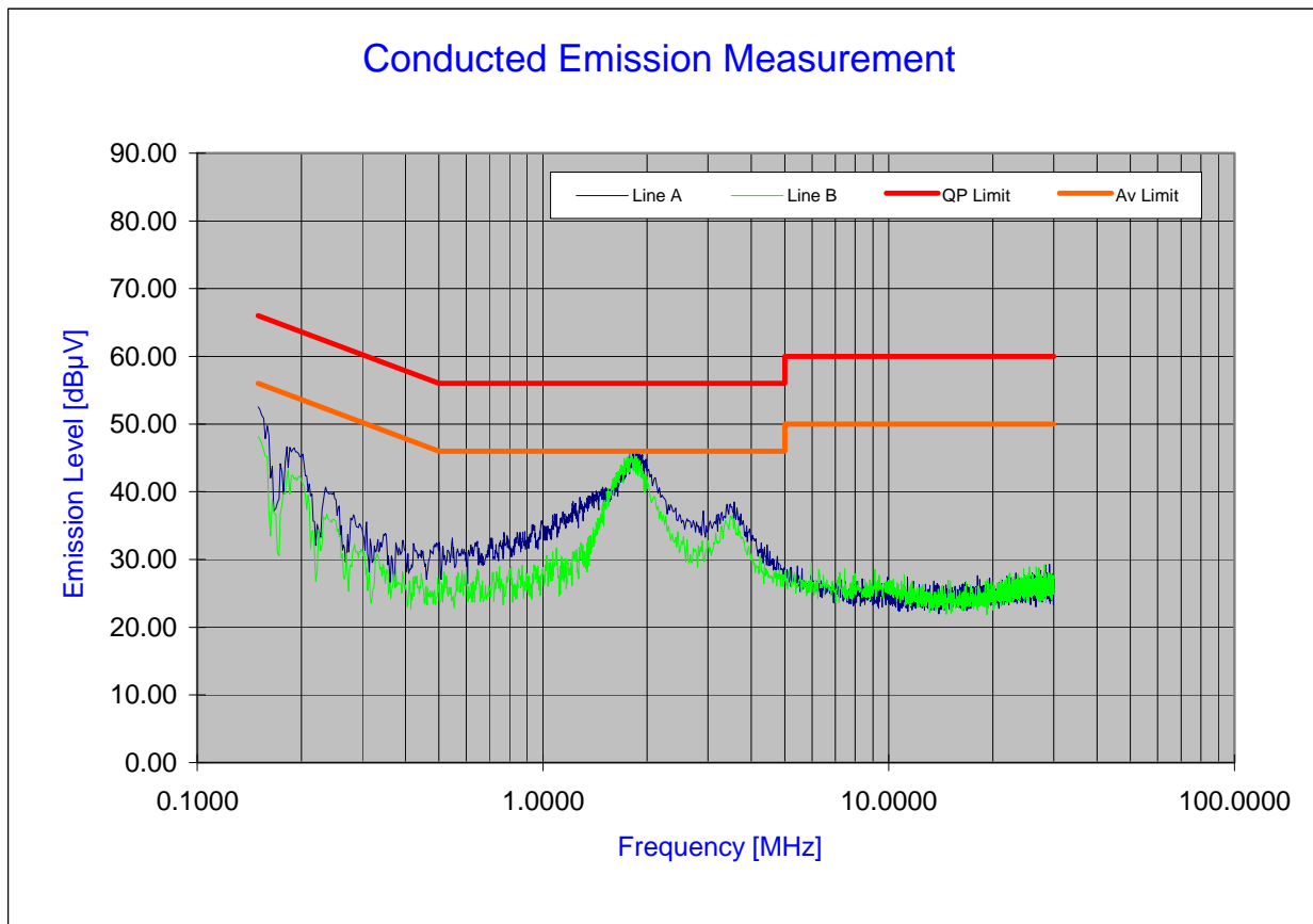
Plot 6-43. Line Conducted Plot with 802.11b
