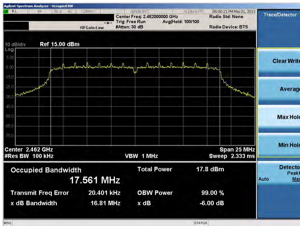
Plot 6-9. 6dB Bandwidth Plot (802.11n LGI (2.4GHz) – Ch. 11)
