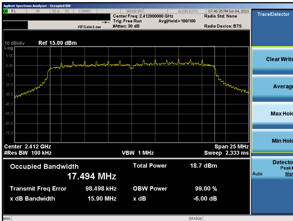
Plot 6-10. 6dB Bandwidth Plot (802.11n SGI (2.4GHz) – Ch. 1)
