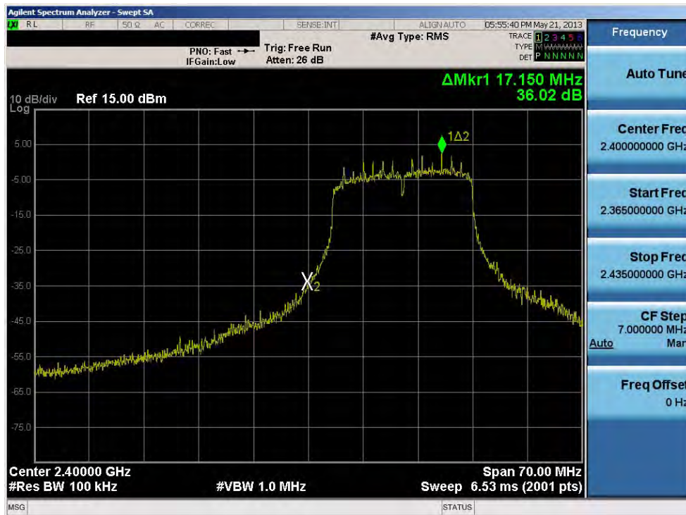
Plot 6-29. Band Edge Plot (802.11n LGI (2.4GHz) – Ch. 1)
