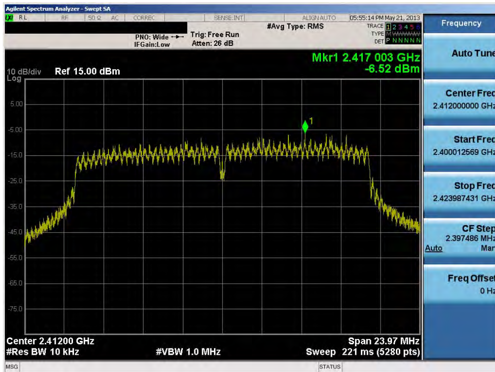
Plot 6-19. Power Spectral Density Plot (802.11n LGI (2.4GHz) – Ch. 1)
