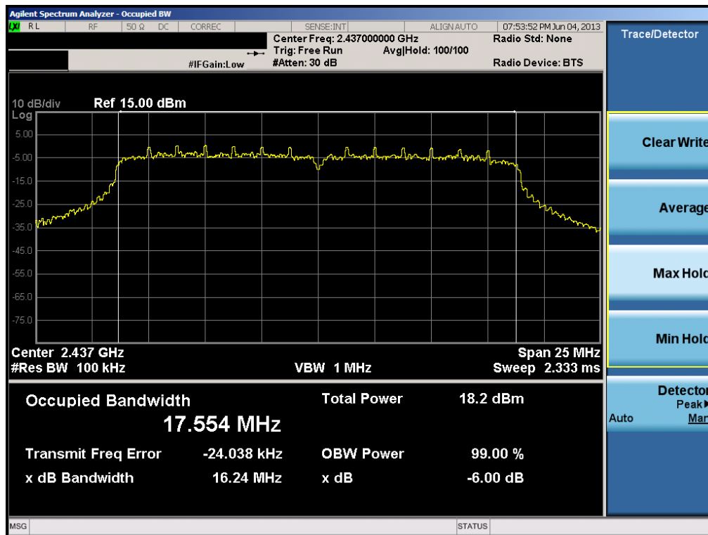
Plot 6-11. 6dB Bandwidth Plot SGI (802.11n (2.4GHz) – Ch. 6)
