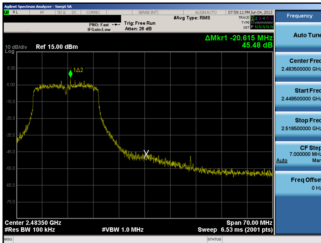
Plot 6-32. Band Edge Plot (802.11n SGI (2.4GHz) – Ch. 11)
