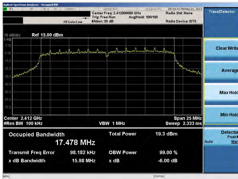
Plot 6-7. 6dB Bandwidth Plot (802.11n LGI (2.4GHz) – Ch. 1)
