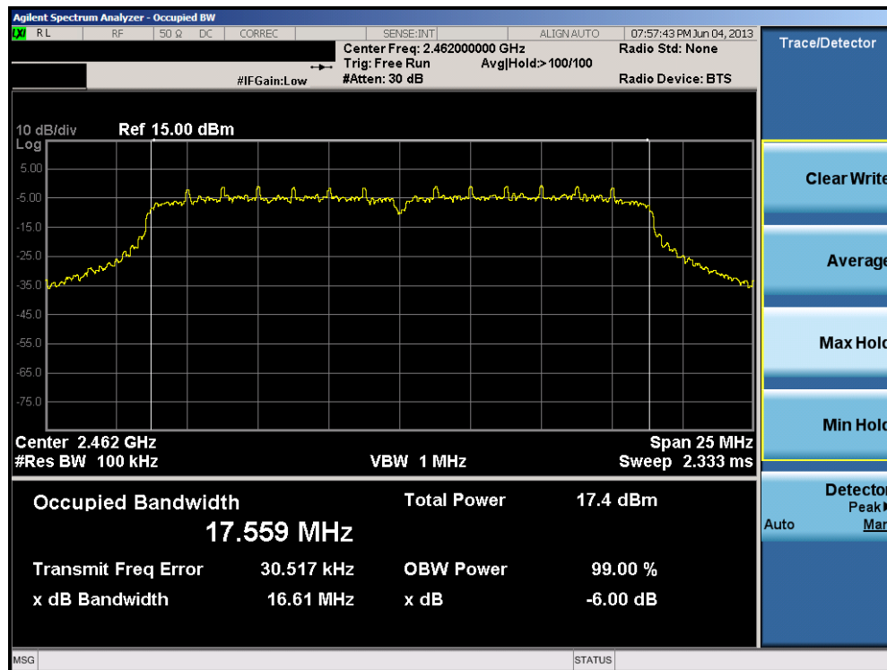
Plot 6-12. 6dB Bandwidth Plot (802.11n SGI (2.4GHz) – Ch. 11)
