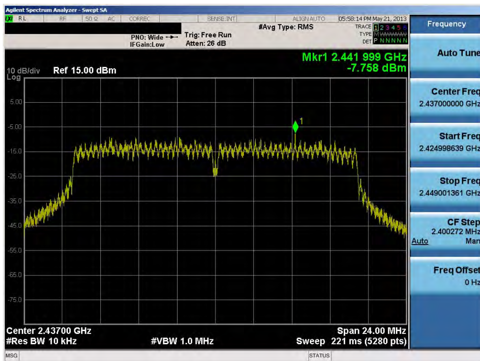
Plot 6-20. Power Spectral Density Plot (802.11n LGI (2.4GHz) – Ch. 6)
