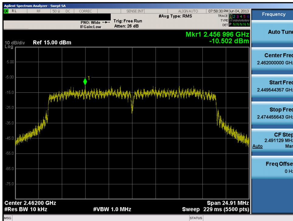
Plot 6-24. Power Spectral Density Plot (802.11n SGI (2.4GHz) – Ch. 11)
