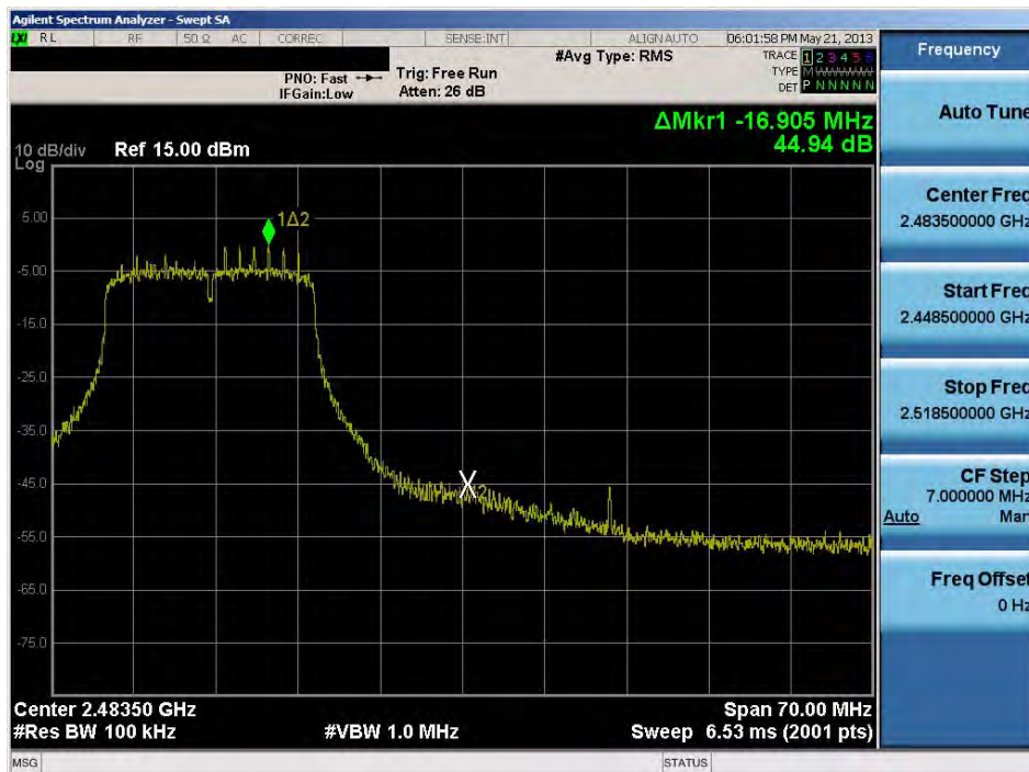
Plot 6-30. Band Edge Plot (802.11n LGI (2.4GHz) – Ch. 11)
