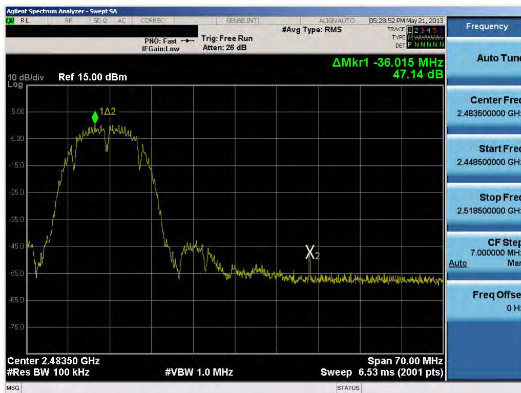
Plot 6-26. Band Edge Plot (802.11b – Ch. 11)
