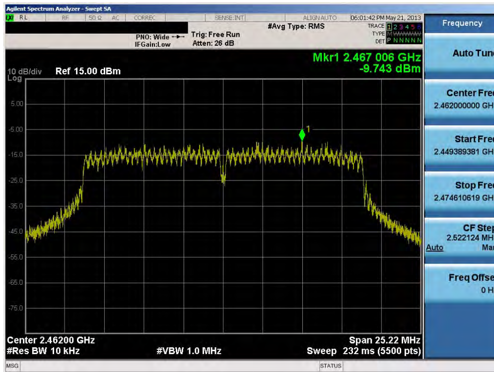
Plot 6-21. Power Spectral Density Plot (802.11n LGI (2.4GHz) – Ch. 11)
