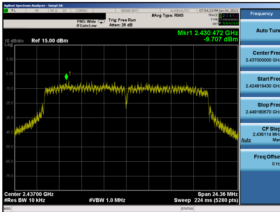
Plot 6-23. Power Spectral Density Plot (802.11n SGI (2.4GHz) – Ch. 6)
