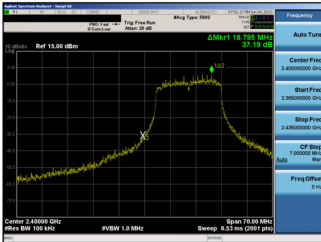
Plot 6-31. Band Edge Plot (802.11n SGI (2.4GHz) – Ch. 1)
