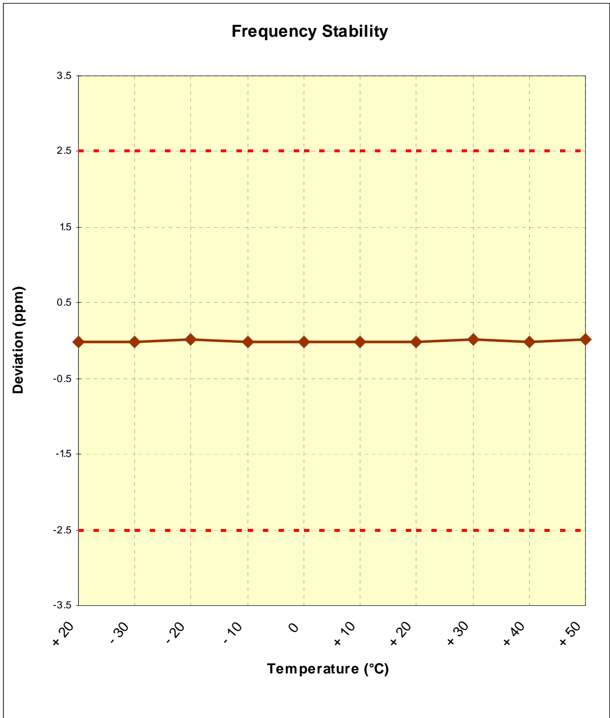
Figure 6-1. Frequency Stability Graph (Cellular WCDMA Mode – Ch. 4183)
