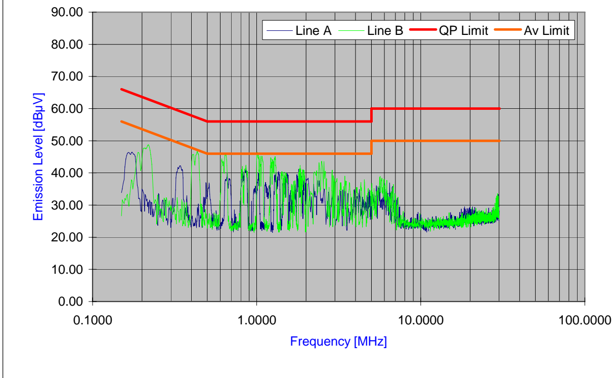
Plot 6-24. Line Conducted Plot with Bluetooth
