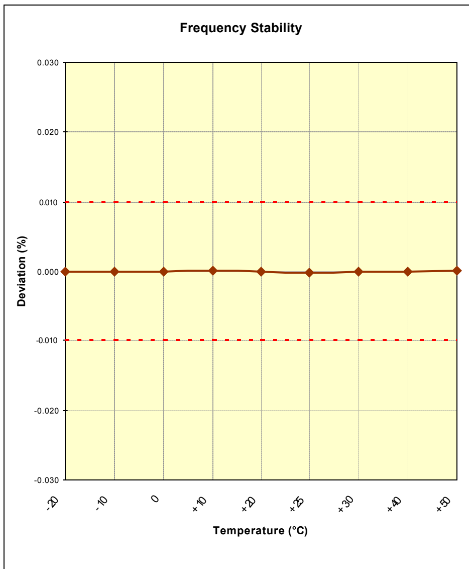
Figure 8-3. Frequency Stability Plot
