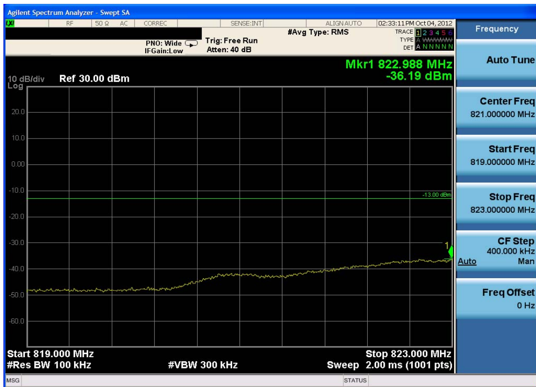
Plot 7-6. 4MHz Span Plot (Cellular WCDMA Mode – Ch. 4132)
