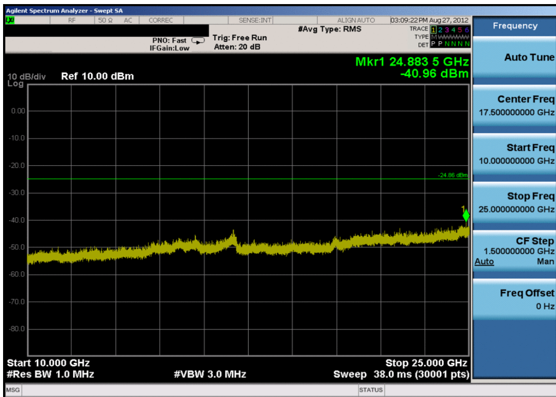
Plot 6-28. Conducted Spurious Plot (Bluetooth, 3Mbps – Ch. 0)
