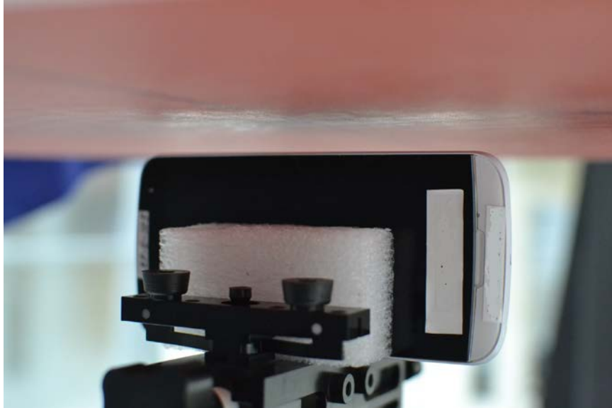
SAR Test Setup Photo 9 - Right Side at 1.0 cm
