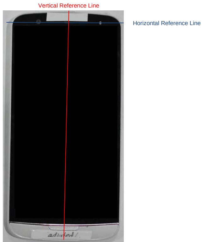
SAR Test Setup Photo 11 - DUT Reference Lines
