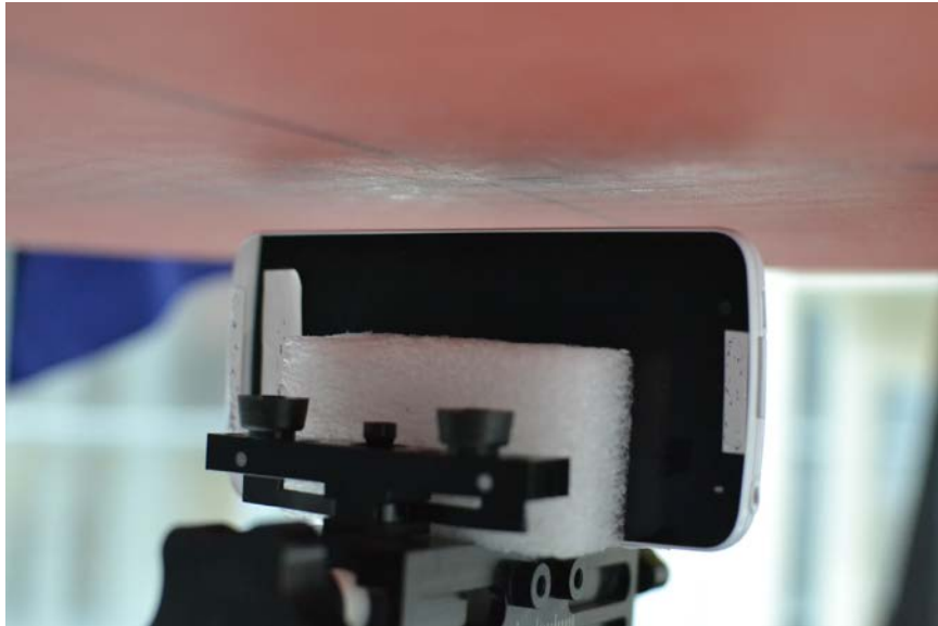
SAR Test Setup Photo 10 - Left Side at 1.0 cm
