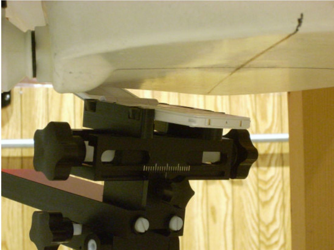
Figure 10: Mouth-Jaw SAR with 3.0 cm Space
