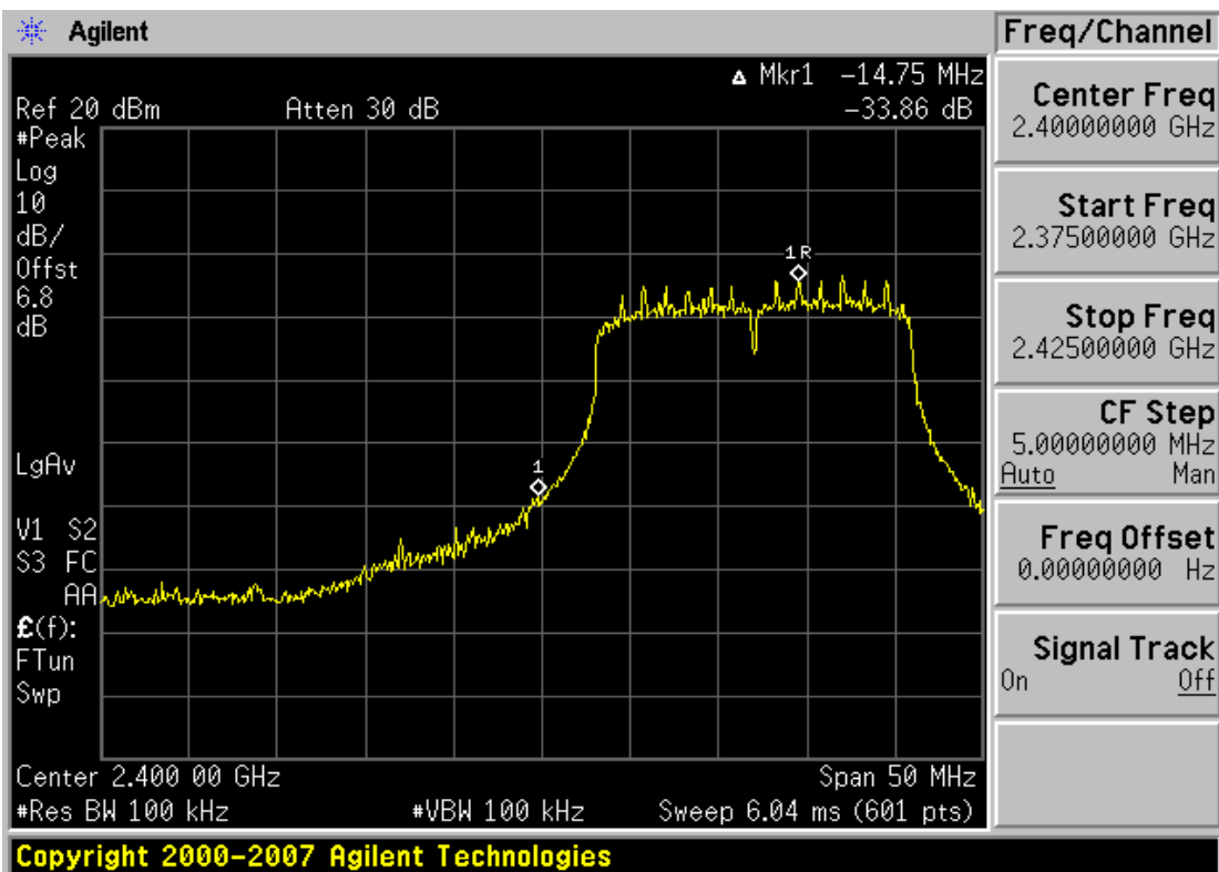
Plot 6-11. Band Edge Plot (802.11n – Ch. 1)
