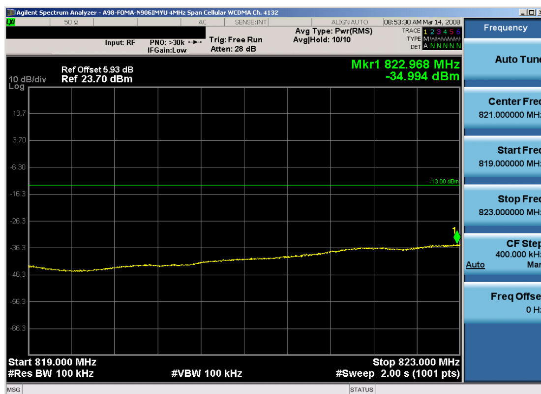
Plot 7-4. 4MHz Span Plot (Cellular WCDMA Mode – Ch. 4132)
