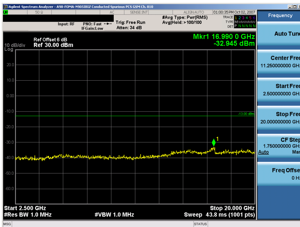
Plot 7-8. Conducted Spurious Plot (PCS GPRS Mode – Ch. 810)
