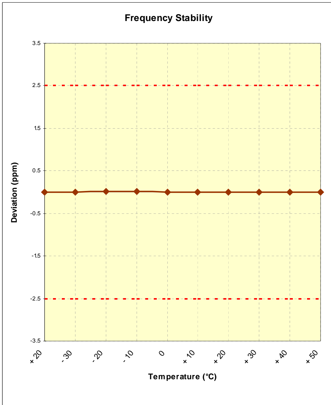
Plot 6-1. Frequency Stability Graph (PCS GPRS Mode – Ch. 661)
