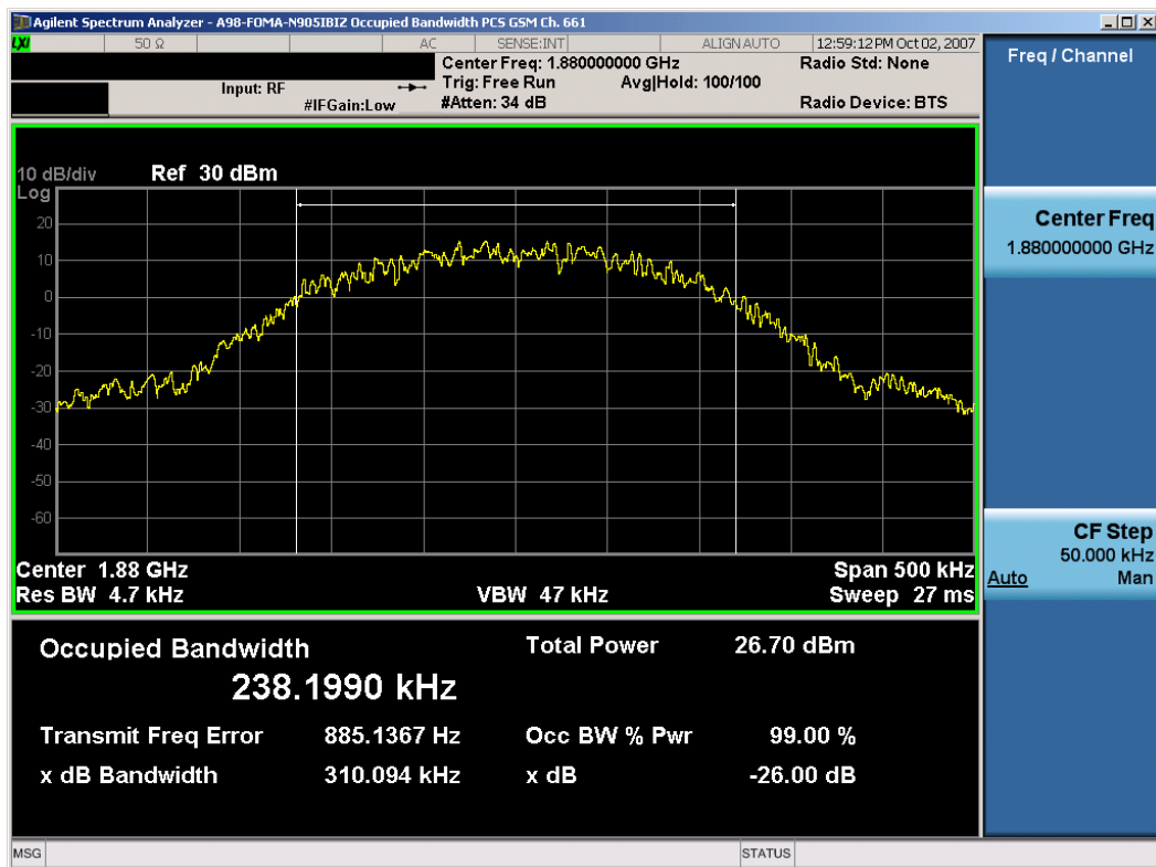
Plot 7-6. Occupied Bandwidth Plot (PCS GPRS Mode – Ch. 661)
