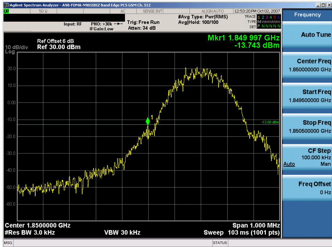
Plot 7-3. Band Edge Plot (PCS GPRS Mode – Ch. 512)
