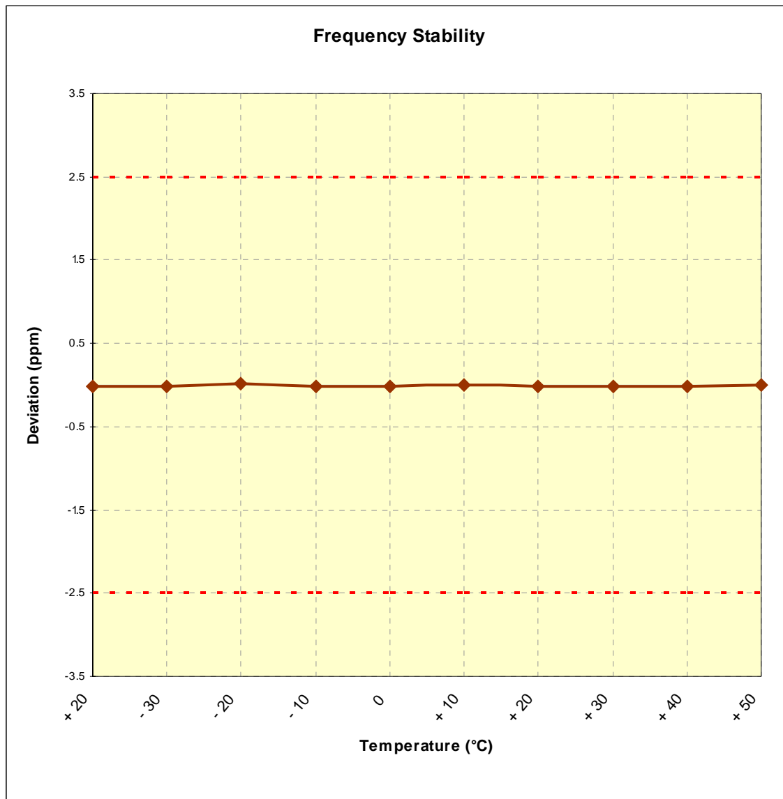
Plot 6-1. Frequency Stability Graph (PCS GSM Mode – Ch. 661)
