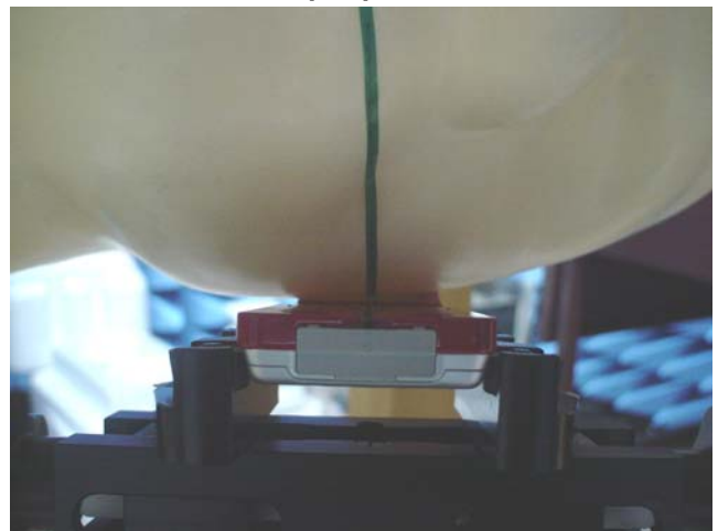
Fig.5 Right Head Section / Ear-Tilt Position(15°)
