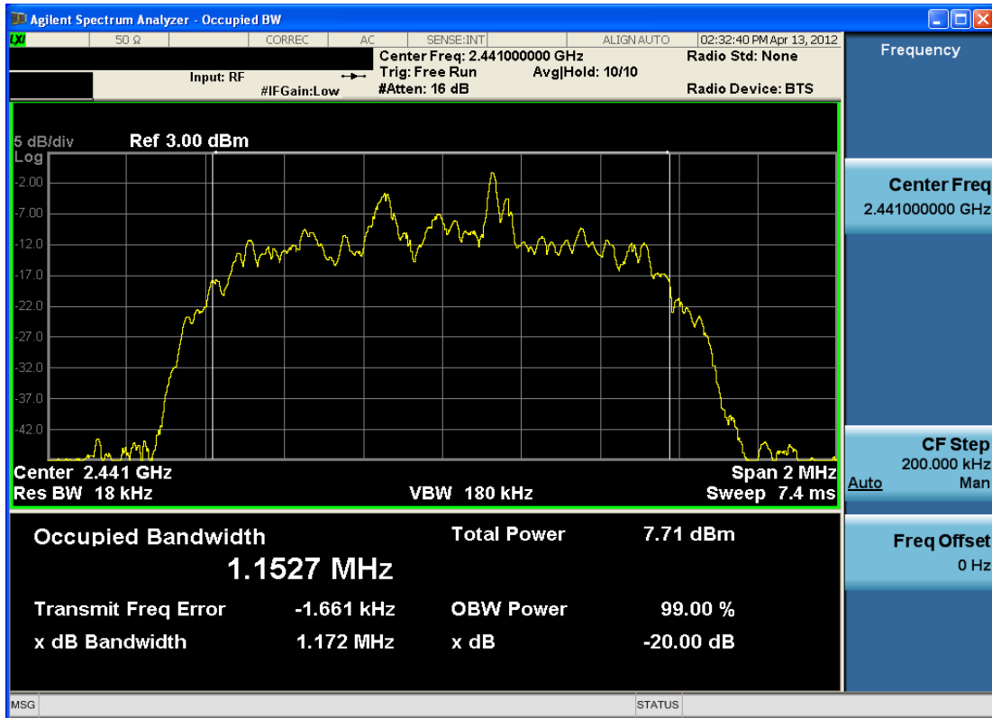
Plot 6-5. 20dB Bandwidth Plot (Bluetooth, 2Mbps – Ch. 39)
