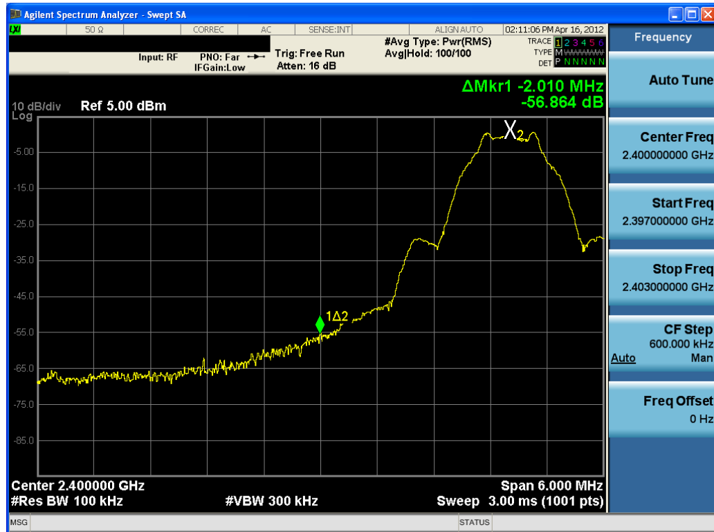
Plot 6-7. Band Edge Plot (Bluetooth LE – Ch. 37)
