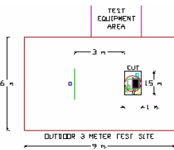
Figure 3-6. Dimensions of Outdoor Test Site
