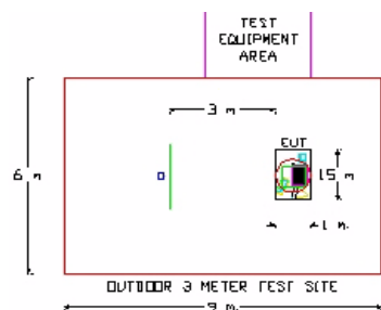
Figure 2-6. Dimensions of Outdoor Test Site
