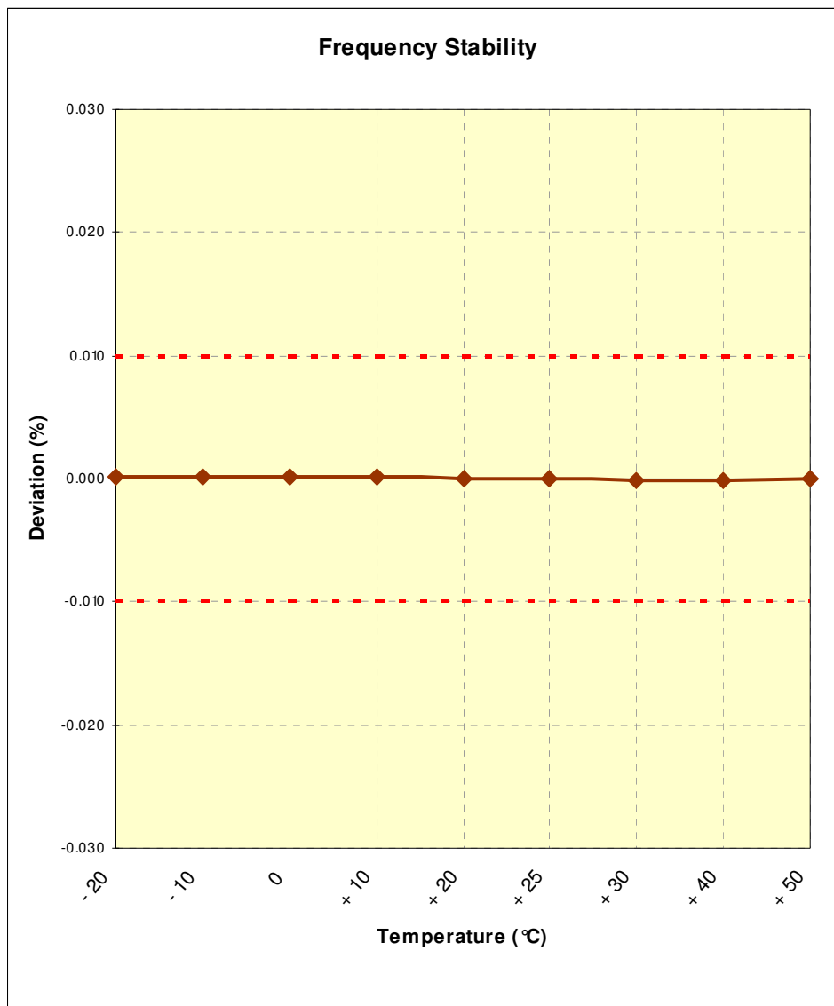
Figure 7-3. Frequency Stability Plot
