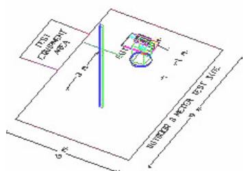
Figure 2-7. Turntable and System Setup
