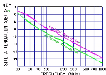
Figure 2-8. Normalized Site Attenuation Curves (H&V)
