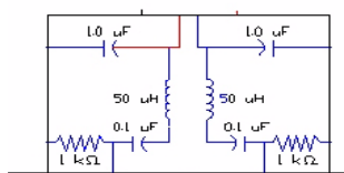
Figure 2-4. LISN Schematic Diagram
