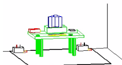
Figure 3-2. Line Conducted Emission Test Set-Up
