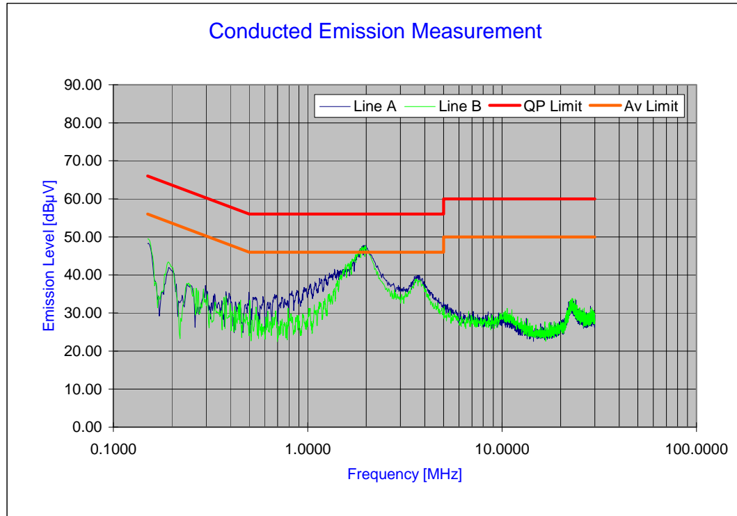
Plot 6-15. Line Conducted Plot with Bluetooth
