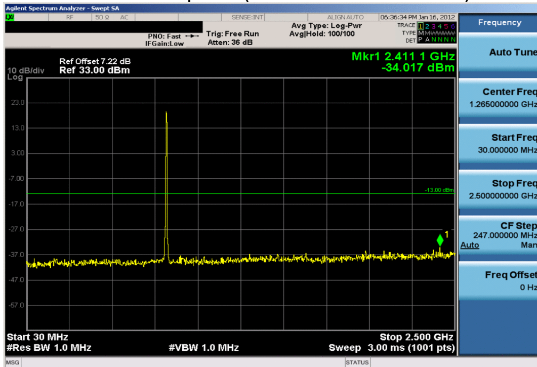
Plot 7-24. Conducted Spurious Plot (Cellular WCDMA Mode – Ch. 4183)
