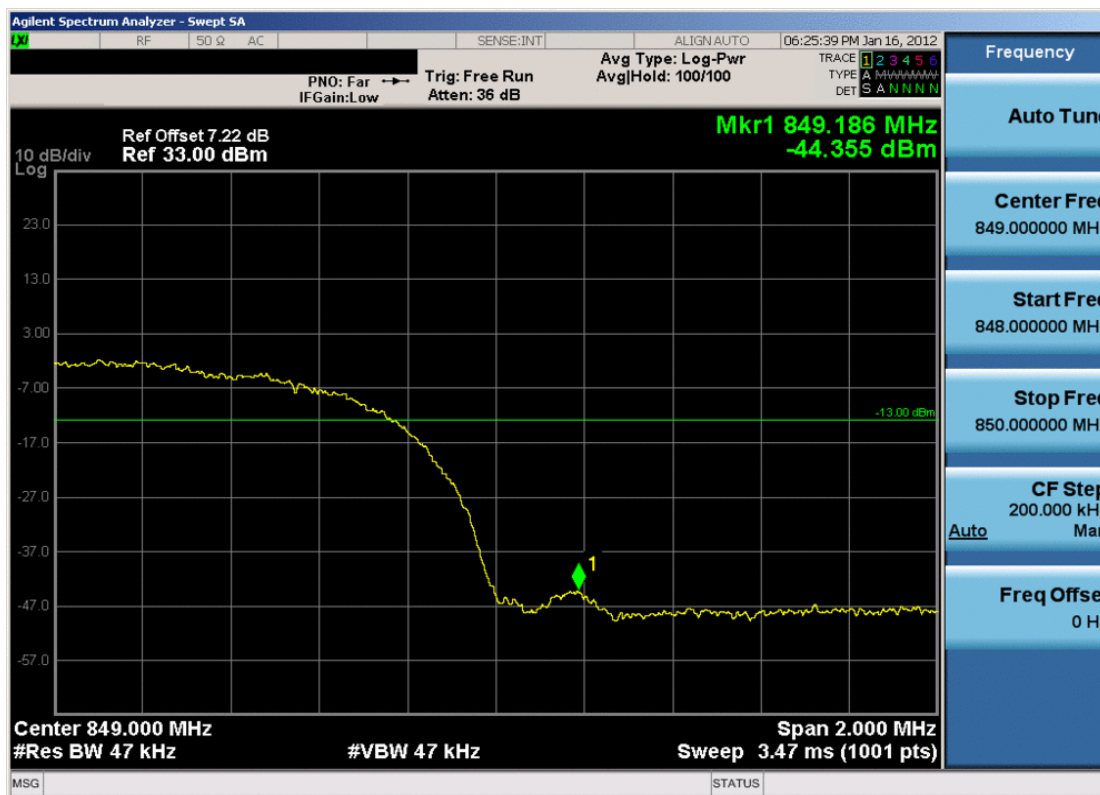
Plot 7-29. Band Edge Plot (Cellular WCDMA Mode – Ch. 4233)
