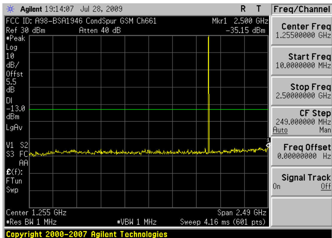
Plot 0-4. Conducted Spurious Plot (PCS GSM Mode – Ch. 661)
