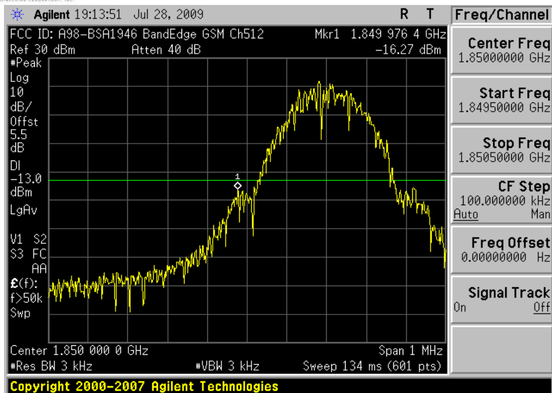
Plot 0-3. Band Edge Plot (PCS GSM Mode – Ch. 512)
