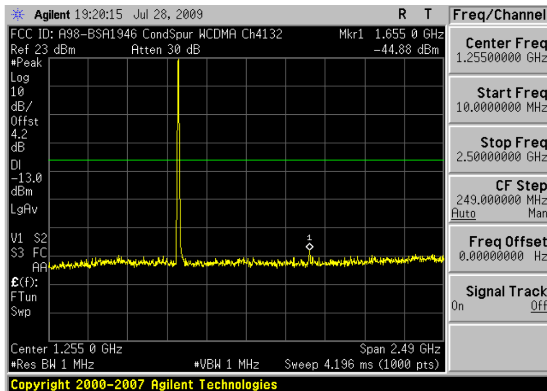
Plot 0-11. Conducted Spurious Plot (Cellular WCDMA Mode – Ch. 4132)
