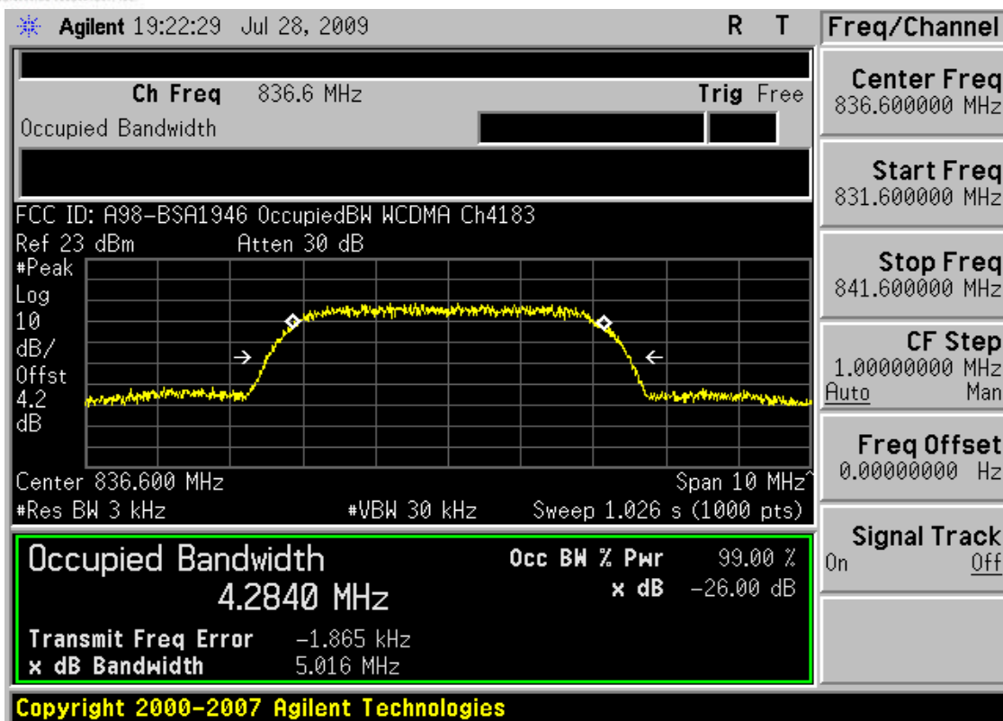
Plot 0-17. Occupied Bandwidth Plot (Cellular WCDMA Mode – Ch. 4183)
