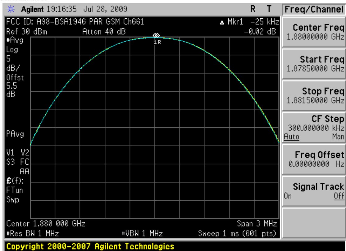
Plot 0-7. Peak-Average Ratio Plot (PCS GSM Mode – Ch. 661)
