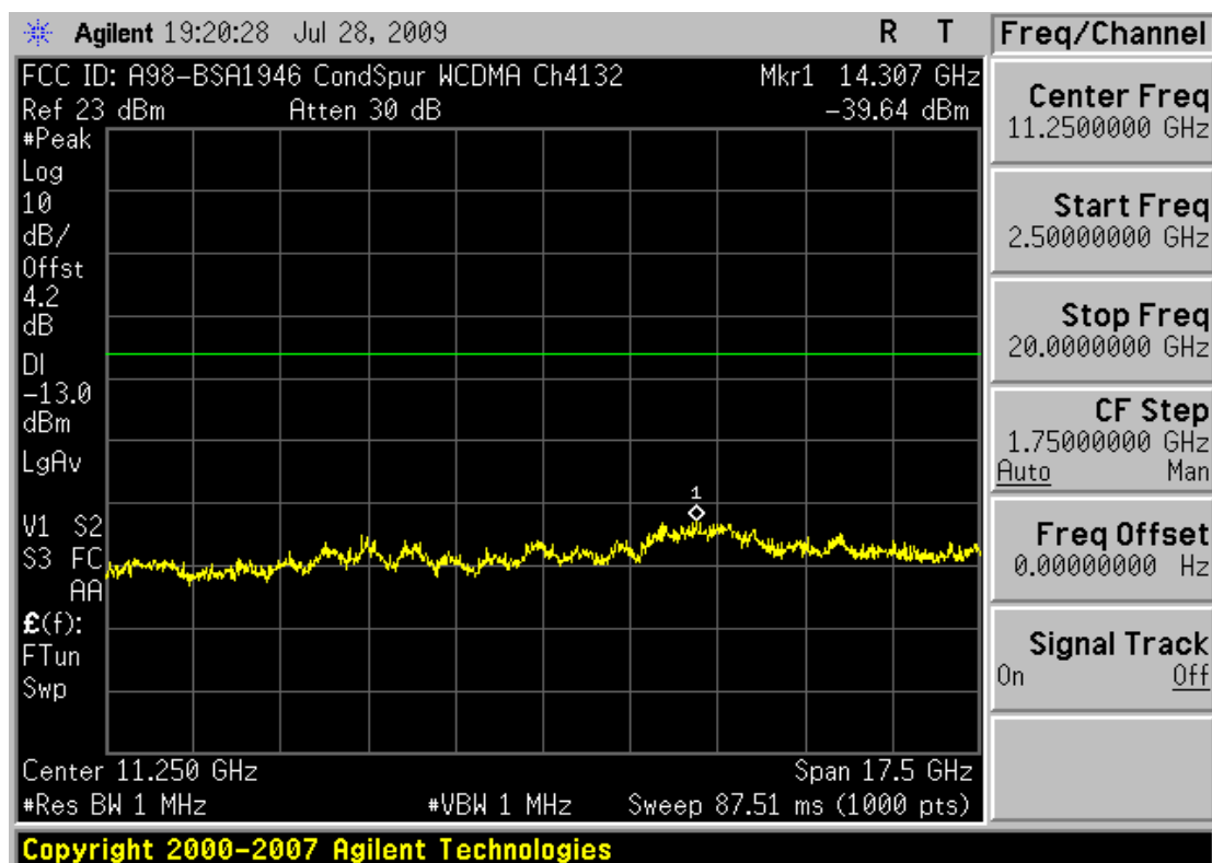
Plot 0-12. Conducted Spurious Plot (Cellular WCDMA Mode – Ch. 4132)
