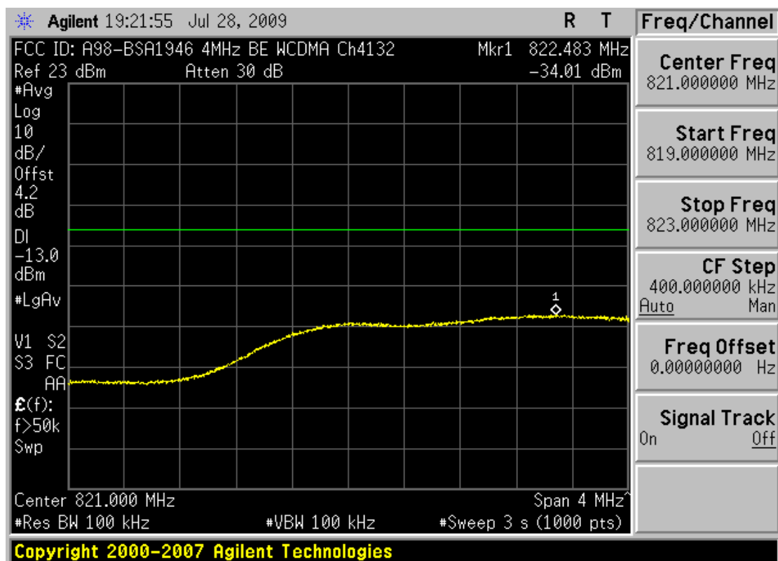
Plot 0-14. 4MHz Span Plot (Cellular WCDMA Mode – Ch. 4132)
