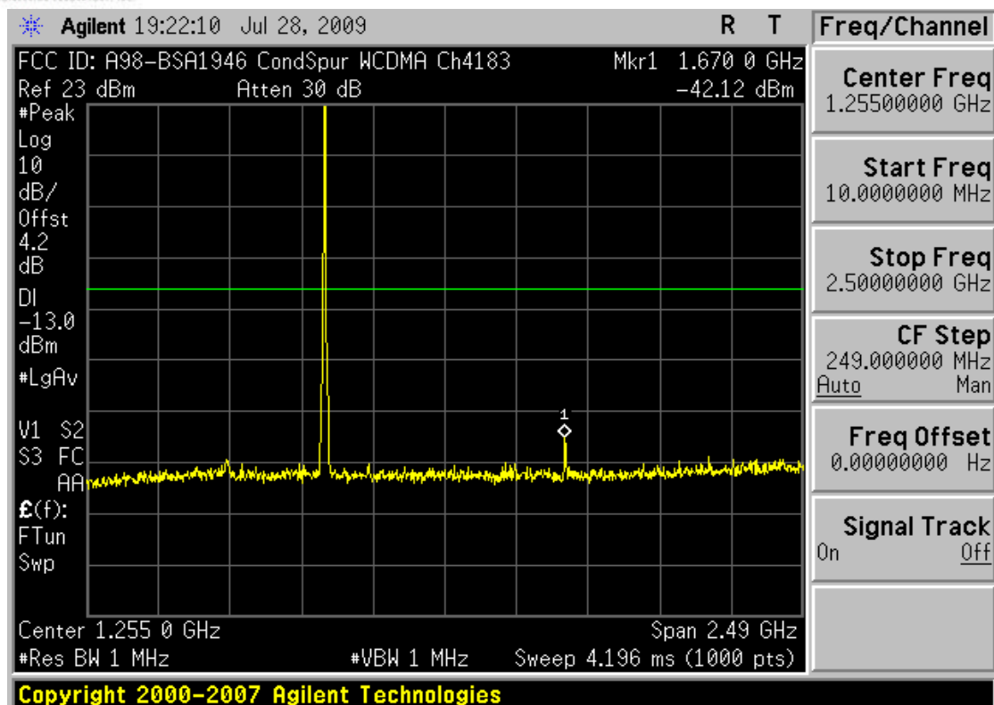
Plot 0-15. Conducted Spurious Plot (Cellular WCDMA Mode – Ch. 4183)
