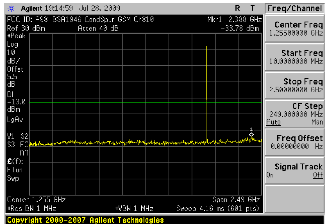
Plot 0-8. Conducted Spurious Plot (PCS GSM Mode – Ch. 810)
