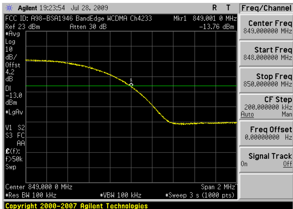
Plot 0-20. Band Edge Plot (Cellular WCDMA Mode – Ch. 4233)
