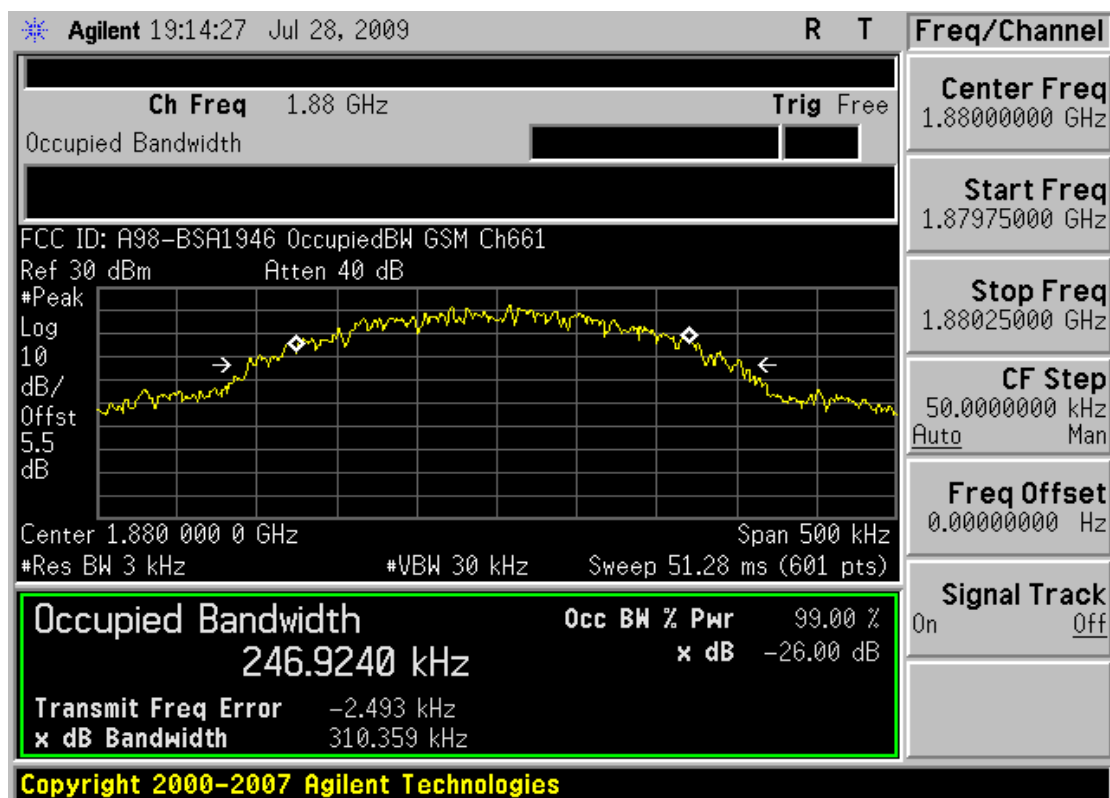
Plot 0-6. Occupied Bandwidth Plot (PCS GSM Mode – Ch. 661)
