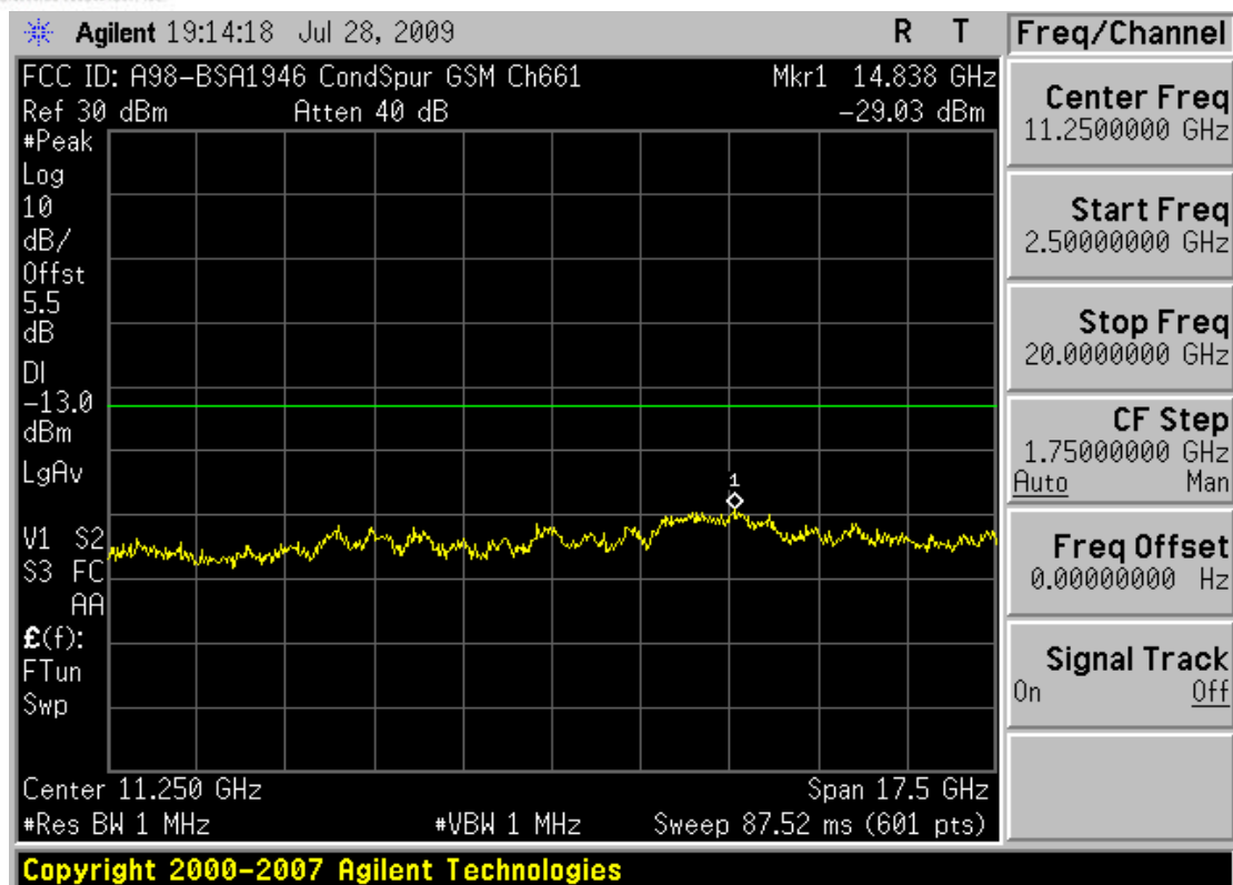
Plot 0-5. Conducted Spurious Plot (PCS GSM Mode – Ch. 661)
