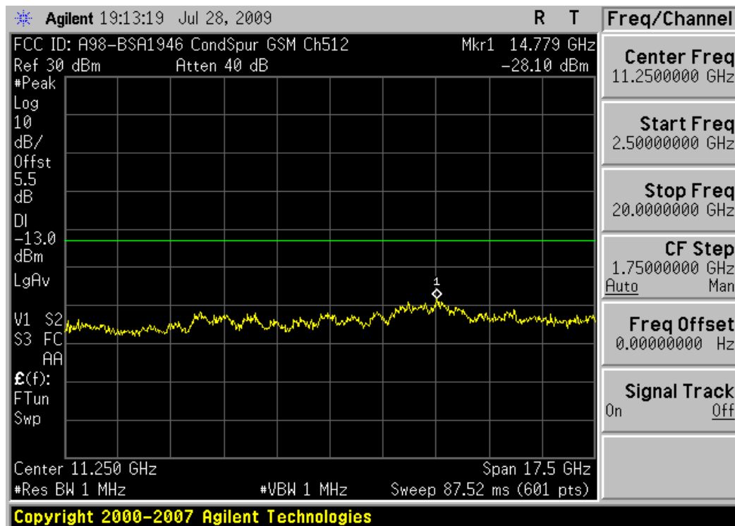
Plot 0-2. Conducted Spurious Plot (PCS GSM Mode – Ch. 512)
