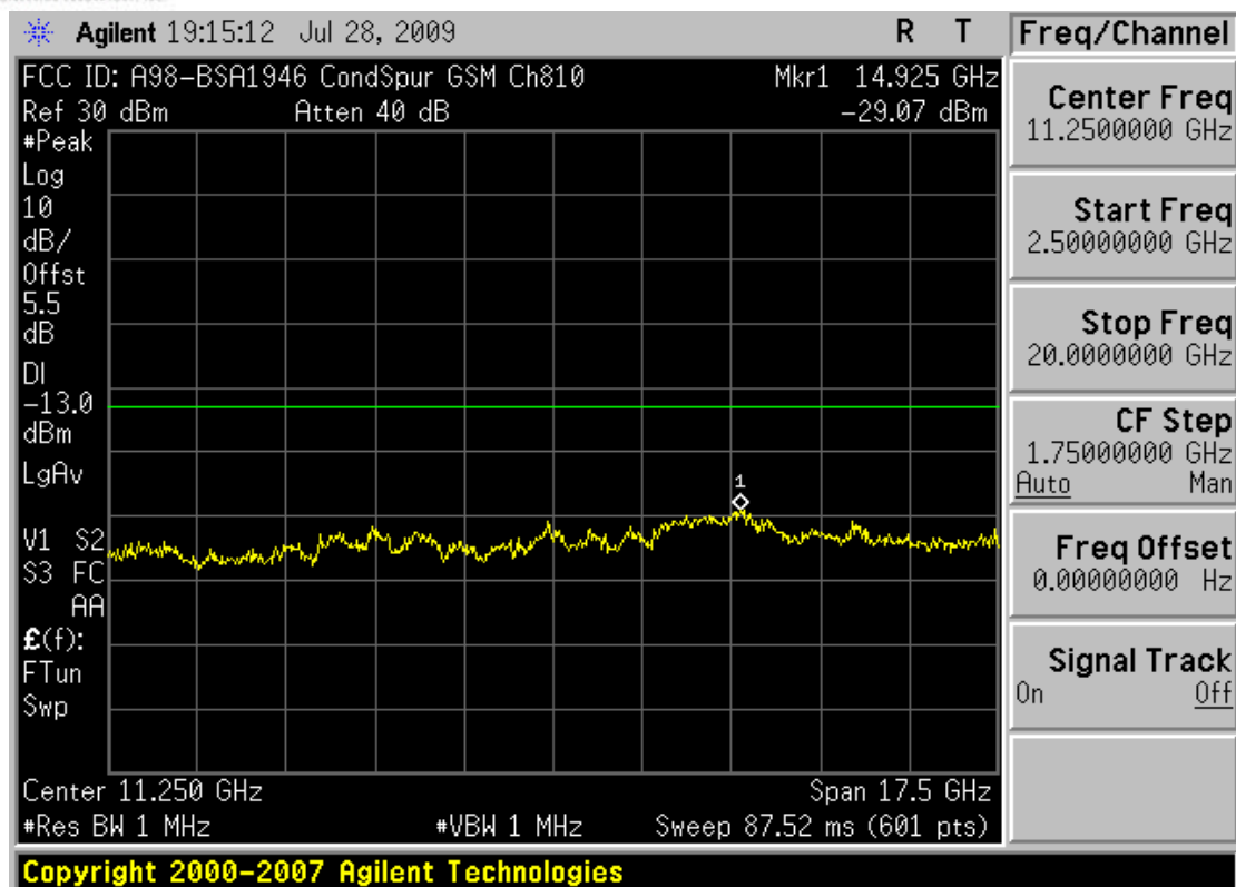
Plot 0-9. Conducted Spurious Plot (PCS GSM Mode – Ch. 810)
