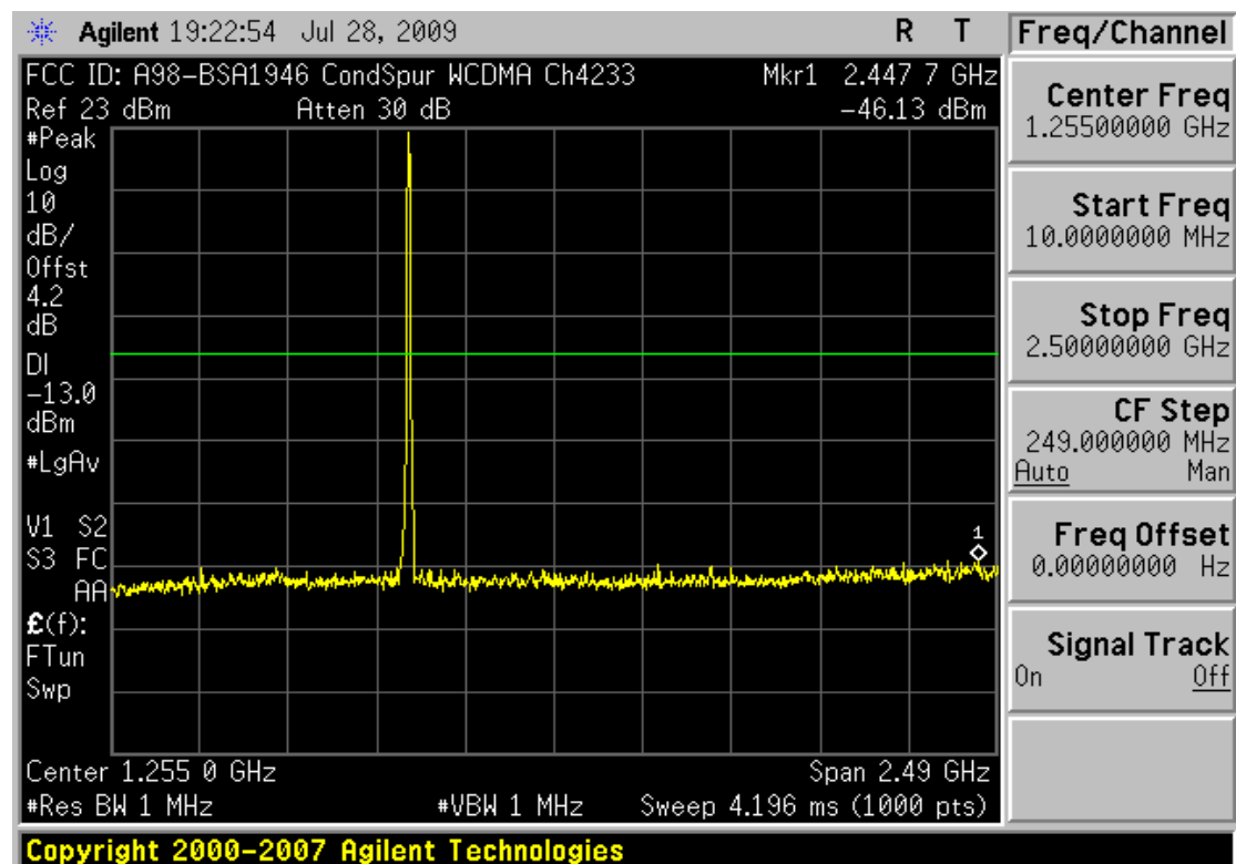
Plot 0-18. Conducted Spurious Plot (Cellular WCDMA Mode – Ch. 4233)
