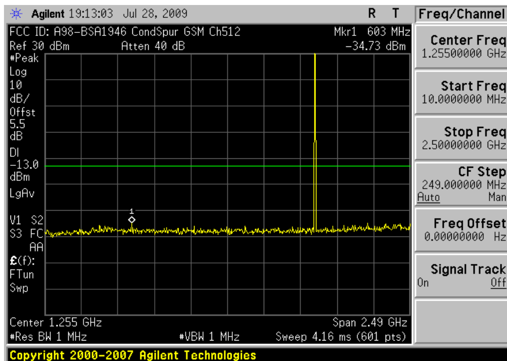
Plot 0-1. Conducted Spurious Plot (PCS GSM Mode – Ch. 512)
