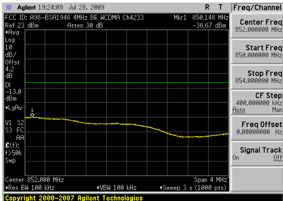
Plot 0-21. 4MHz Span Plot (Cellular WCDMA Mode – Ch. 4233)
