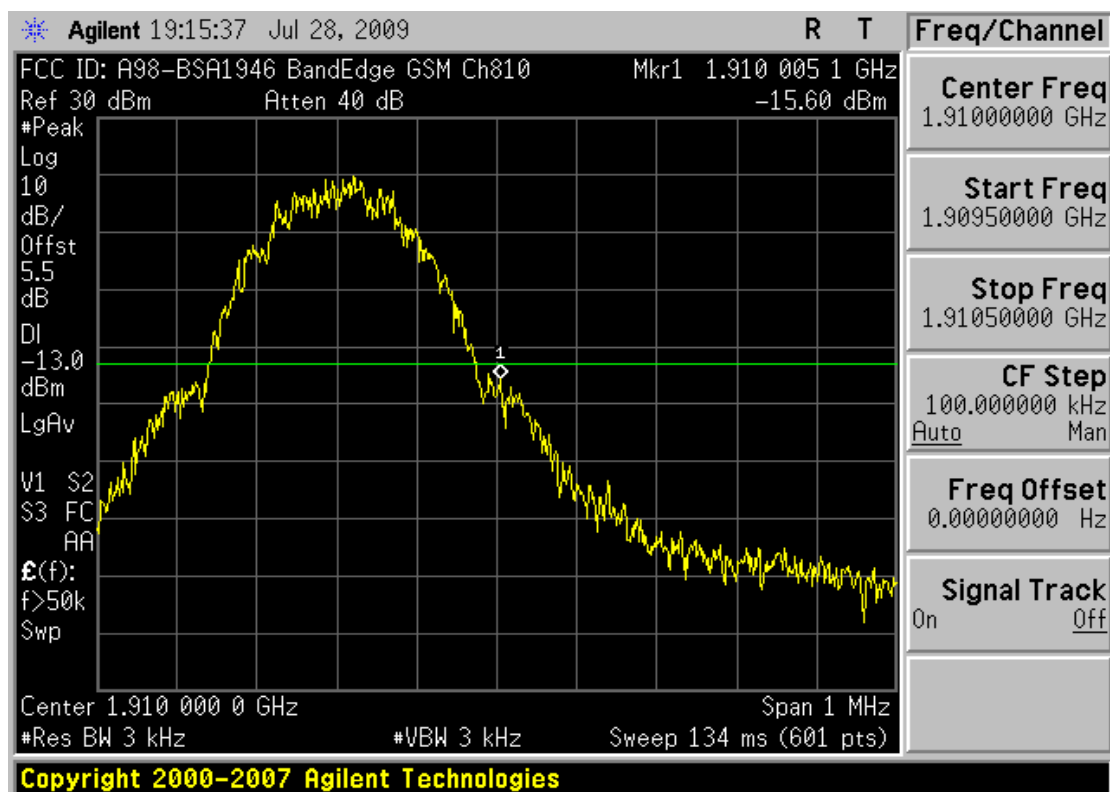
Plot 0-10. Band Edge Plot (PCS GSM Mode – Ch. 810)
