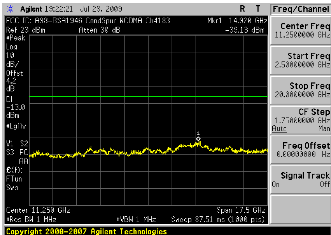
Plot 0-16. Conducted Spurious Plot (Cellular WCDMA Mode – Ch. 4183)
