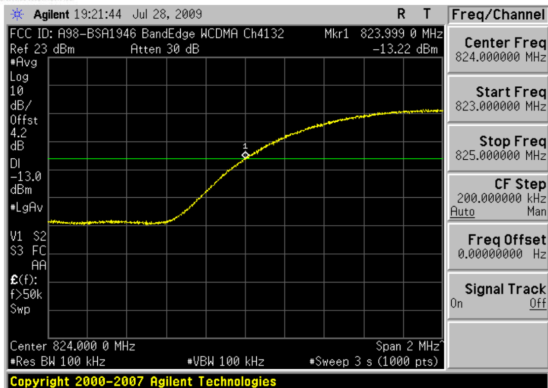
Plot 0-13. Band Edge Plot (Cellular WCDMA Mode – Ch. 4132)
