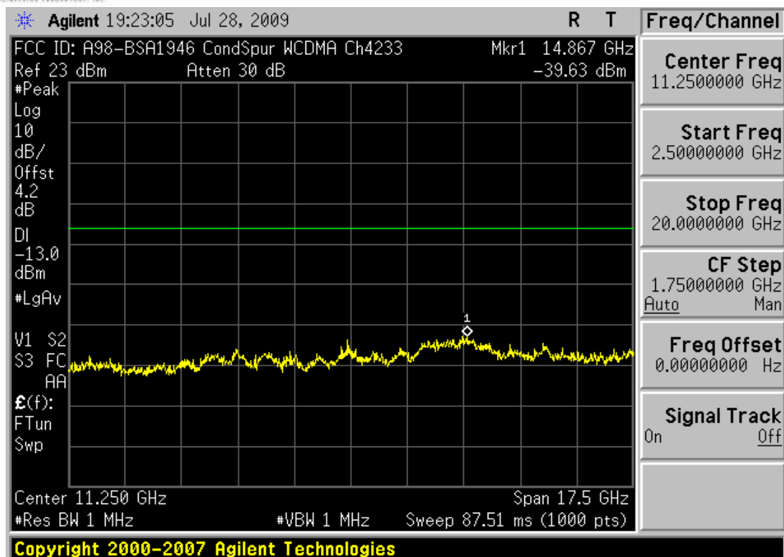
Plot 0-19. Conducted Spurious Plot (Cellular WCDMA Mode – Ch. 4233)
