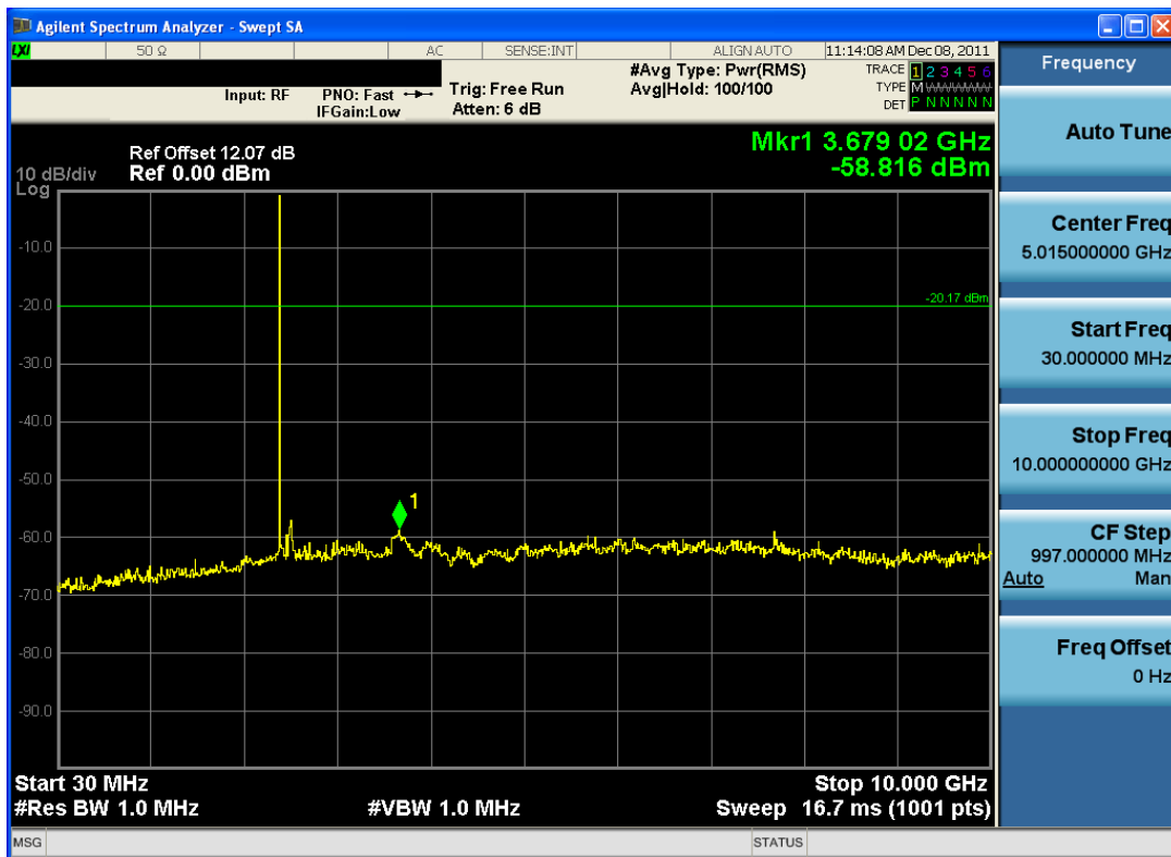
Plot 6-11. Conducted Spurious Plot (Bluetooth LE – Ch. 17)
