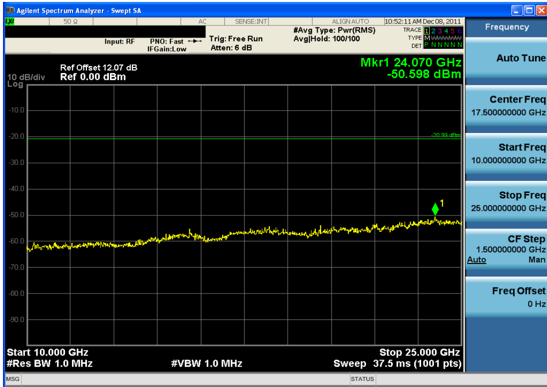
Plot 6-10. Conducted Spurious Plot (Bluetooth LE – Ch. 37)
