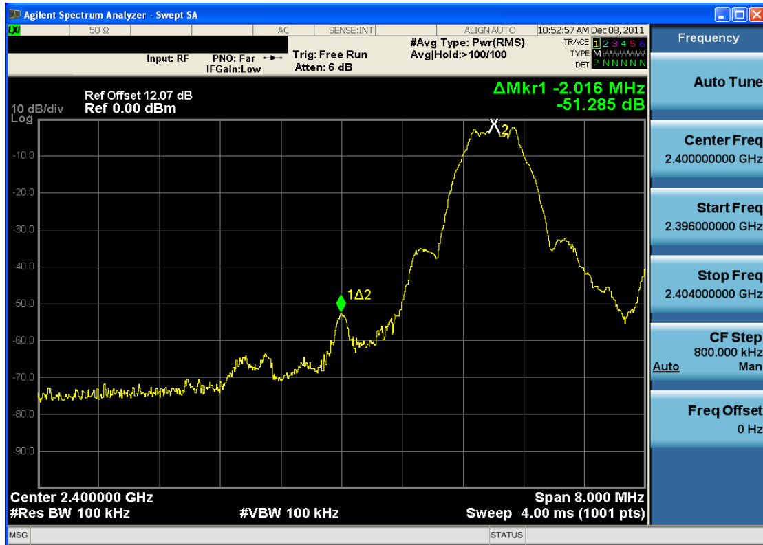
Plot 6-7. Band Edge Plot (Bluetooth LE – Ch. 37)
