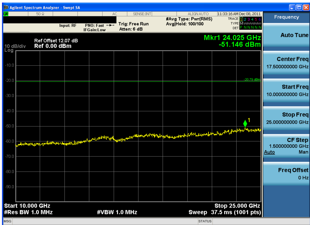
Plot 6-14. Conducted Spurious Plot (Bluetooth LE – Ch. 39)
