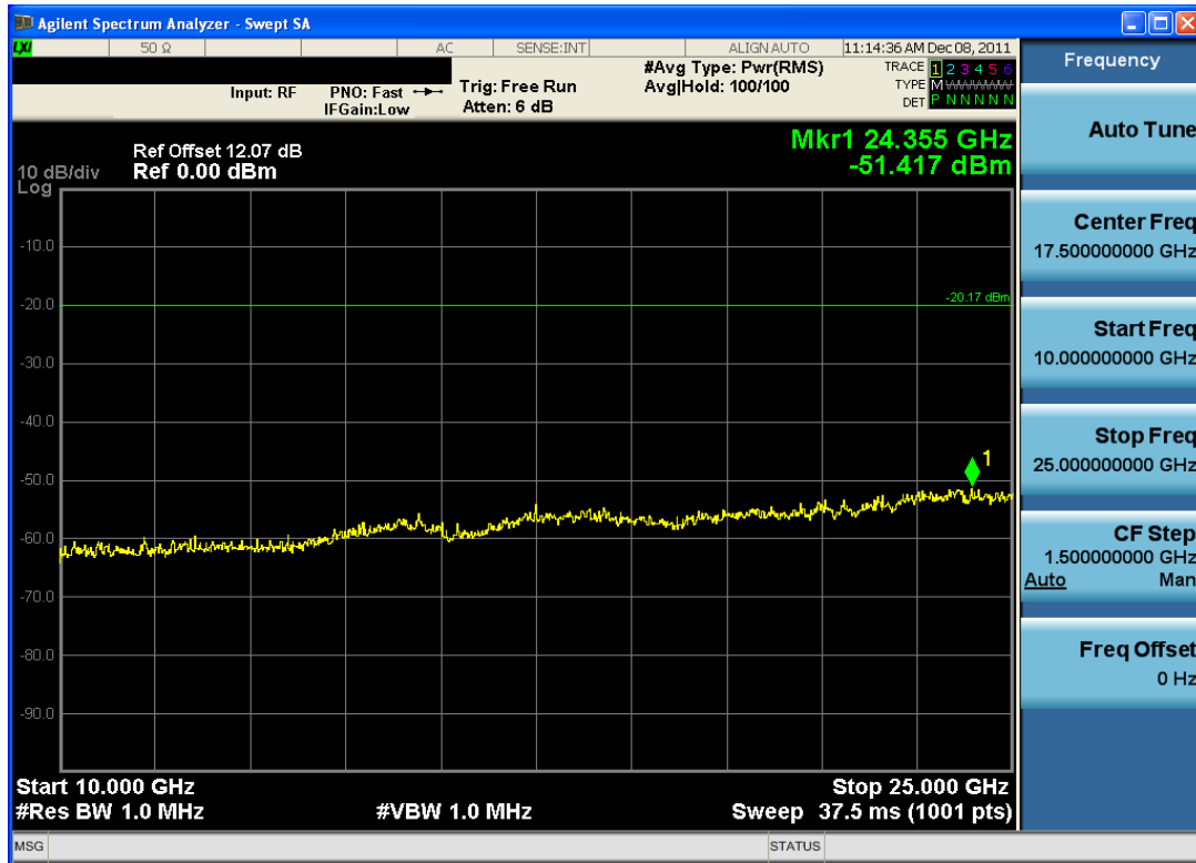
Plot 6-12. Conducted Spurious Plot (Bluetooth LE – Ch. 17)
