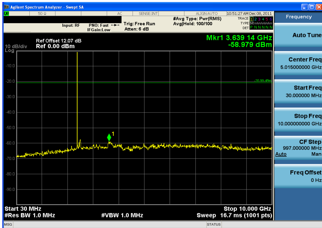
Plot 6-9. Conducted Spurious Plot (Bluetooth LE – Ch. 37)
