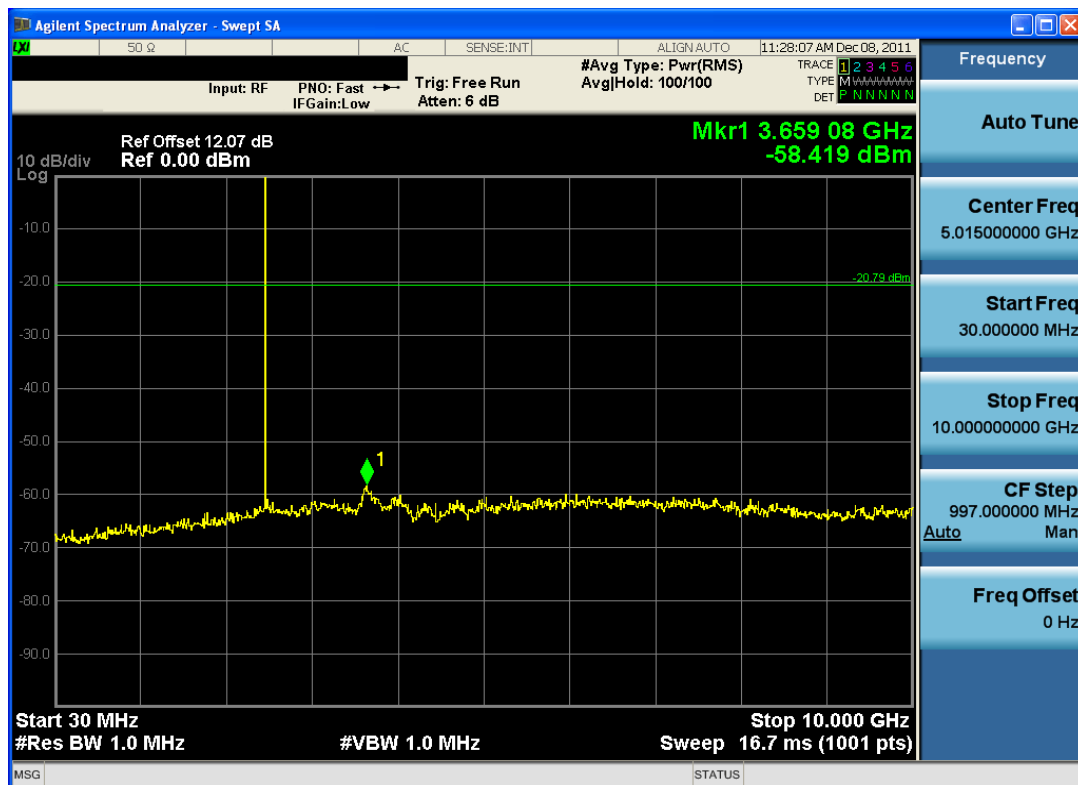
Plot 6-13. Conducted Spurious Plot (Bluetooth LE – Ch. 39)
