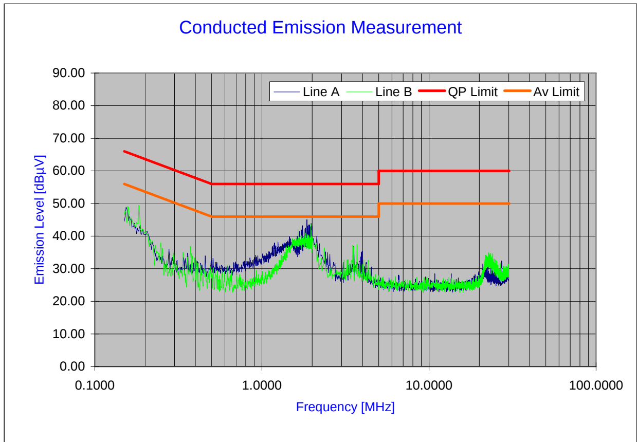
Plot 6-15. Line Conducted Plot with Bluetooth
