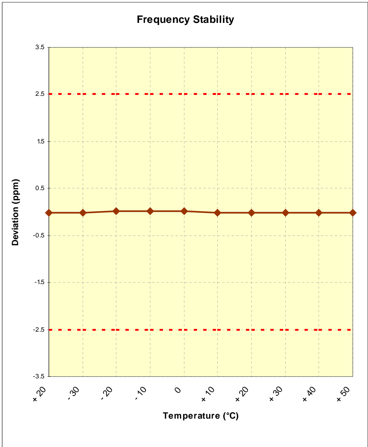
Figure 6-2. Frequency Stability Graph (Cellular WCDMA Mode – Ch. 4183)
