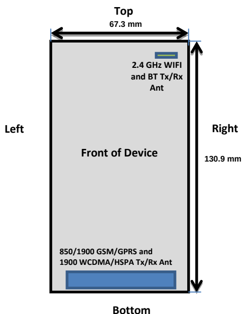
Figure 13-1 Identification of Sides for SAR Testing
