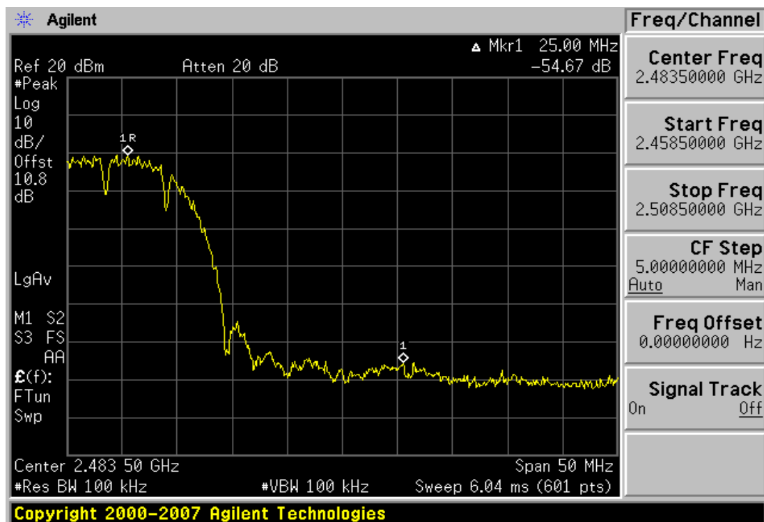
Plot 6-14. Band Edge Plot (802.11b – Ch. 11)
