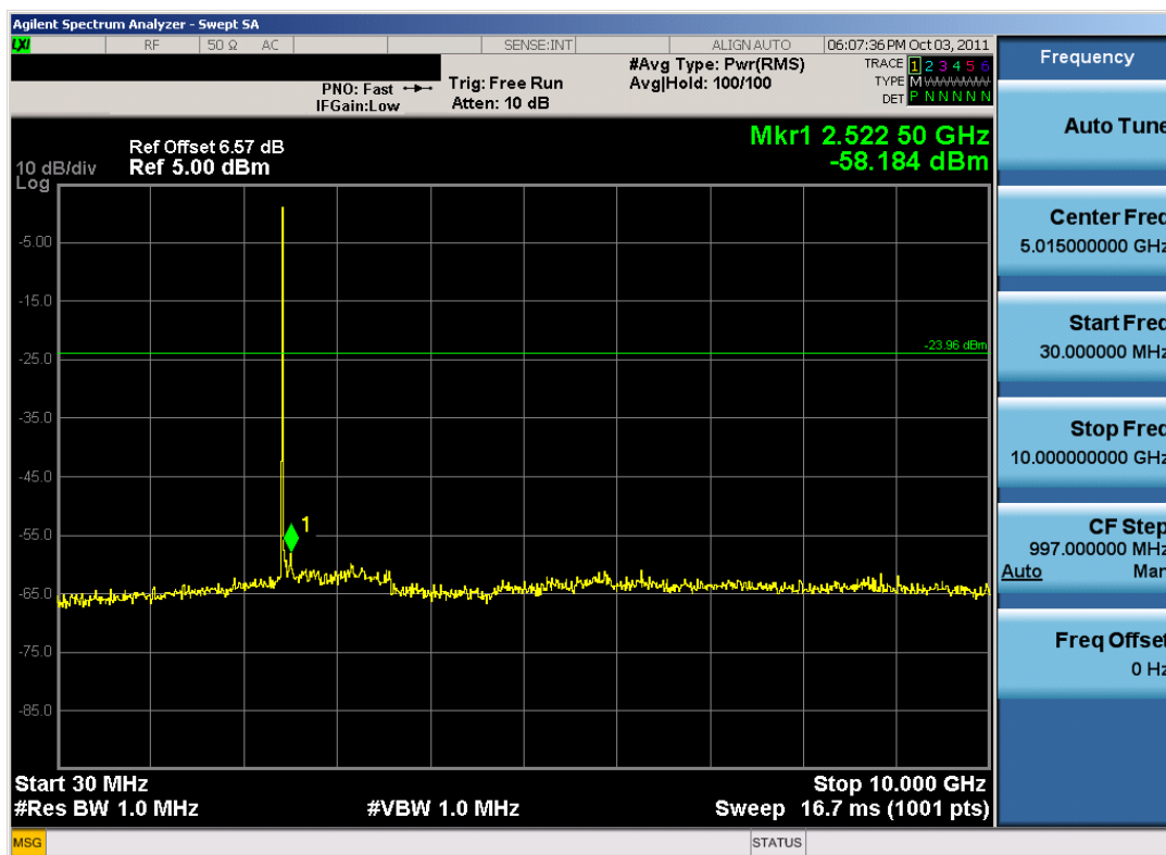
Plot 6-18. Conducted Spurious Plot (Bluetooth, 3Mbps – Ch. 39)
