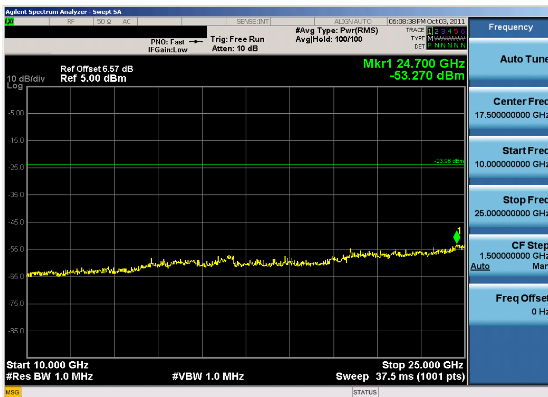
Plot 6-19. Conducted Spurious Plot (Bluetooth, 3Mbps – Ch. 39)
