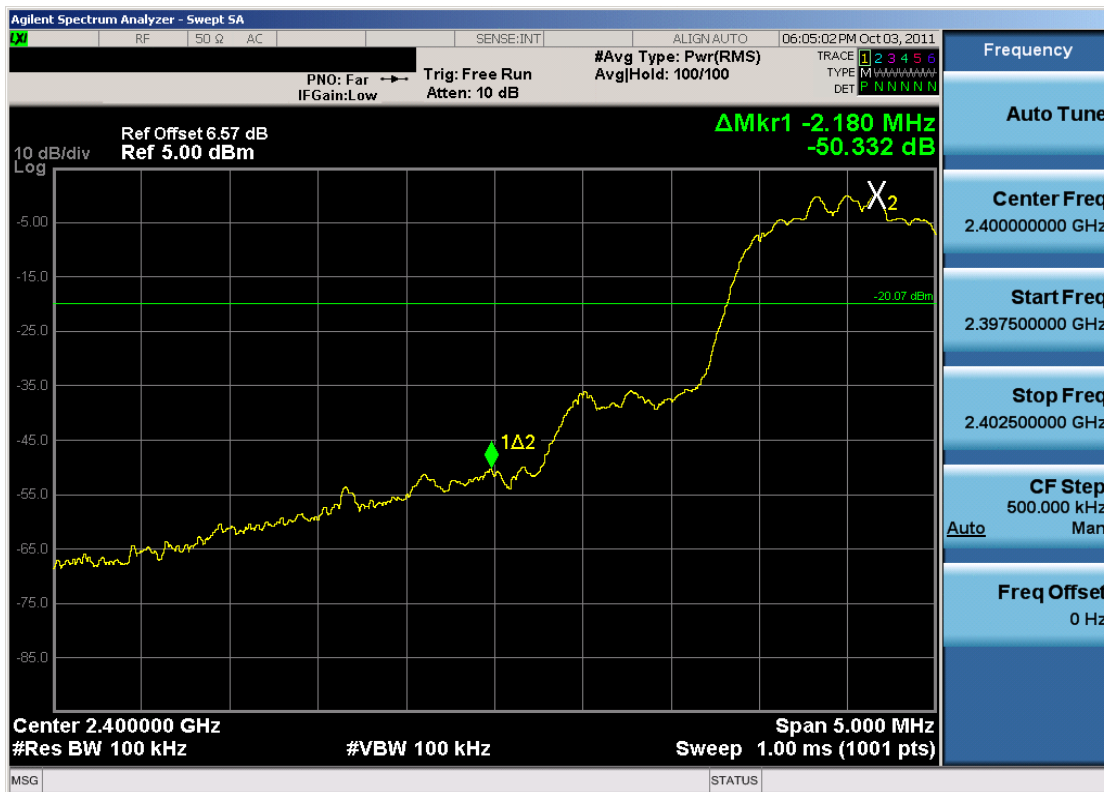
Plot 6-10. Band Edge Plot (Bluetooth, 3Mbps – Ch. 0)
