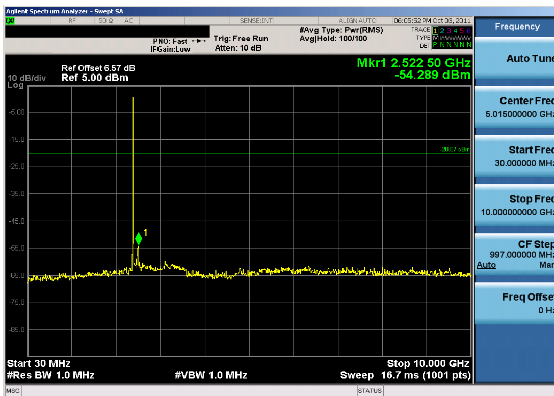
Plot 6-16. Conducted Spurious Plot (Bluetooth, 3Mbps – Ch. 0)
