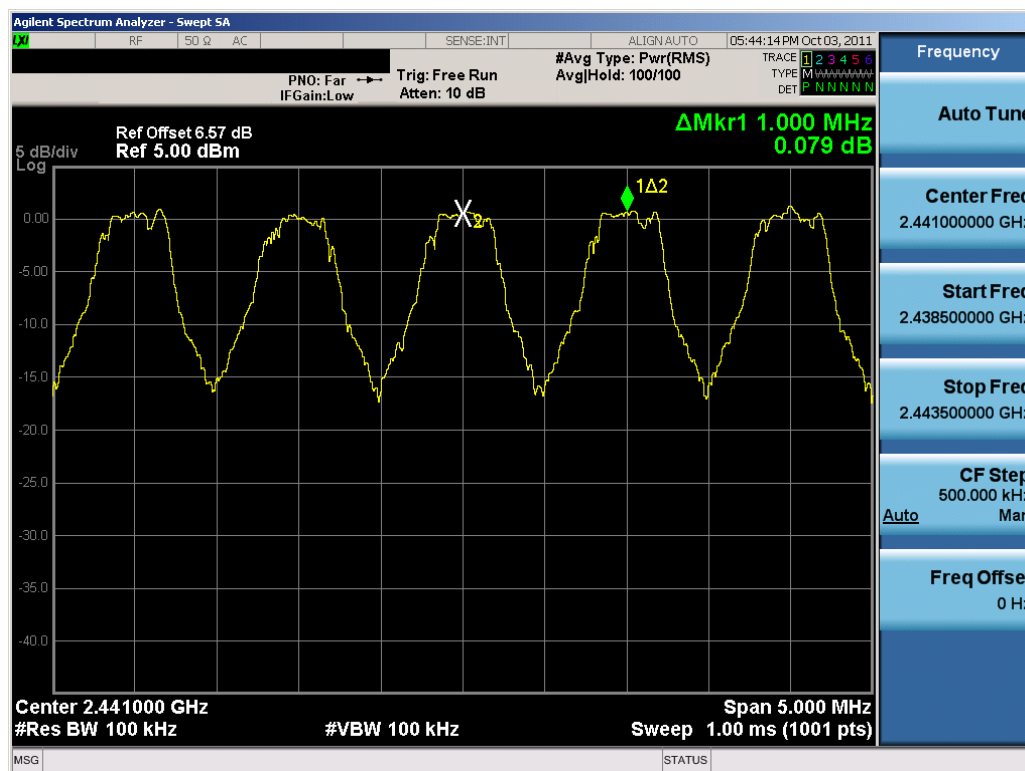
Plot 6-12. Channel Spacing Plot (Bluetooth)
