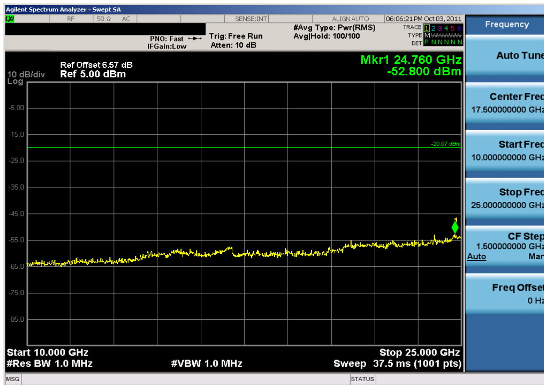
Plot 6-17. Conducted Spurious Plot (Bluetooth, 3Mbps – Ch. 0)
