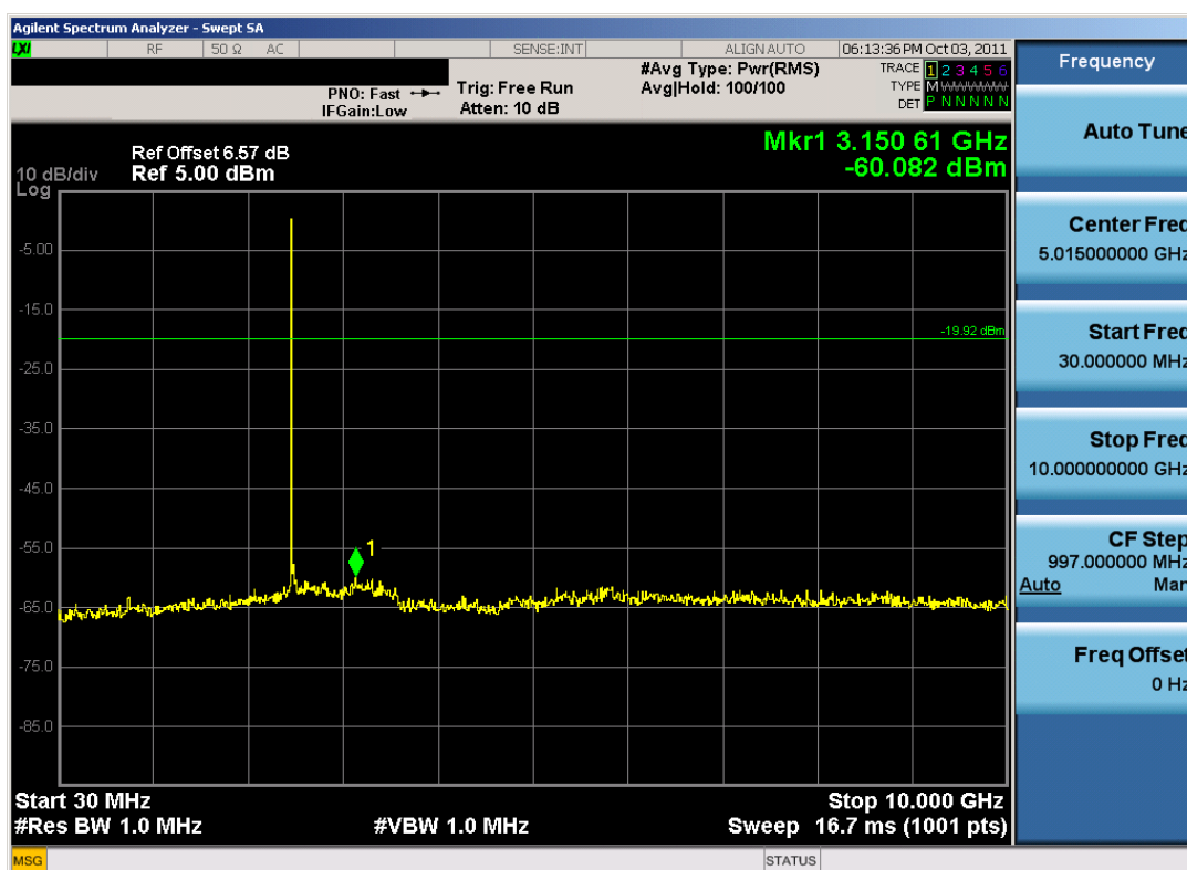
Plot 6-20. Conducted Spurious Plot (Bluetooth, 3Mbps – Ch. 78)
