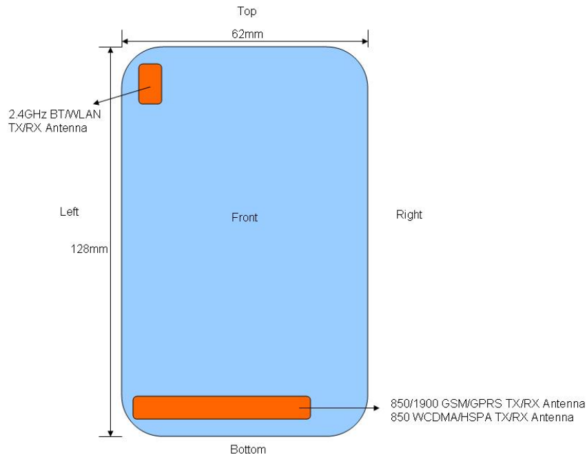
Figure 13-1 Identification of Sides for SAR Testing
