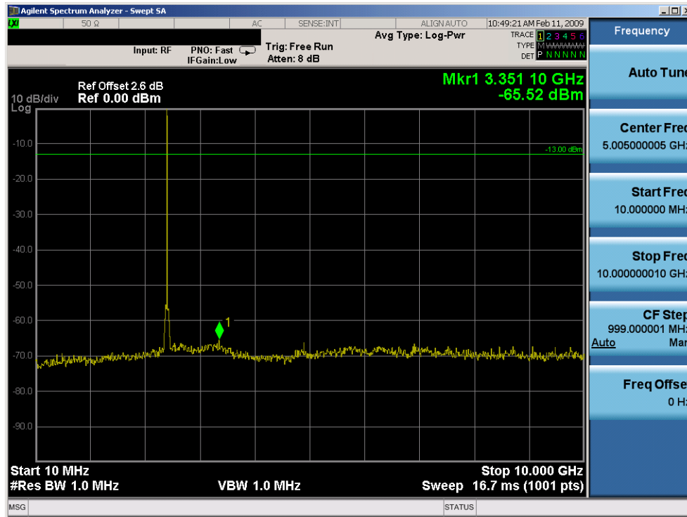
Plot 6-12. Conducted Spurious Plot (Bluetooth – Ch. 0)
