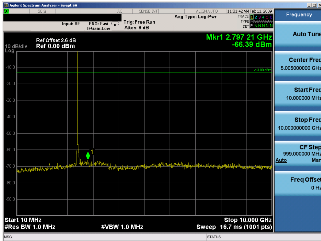
Plot 6-14. Conducted Spurious Plot (Bluetooth – Ch. 39)
