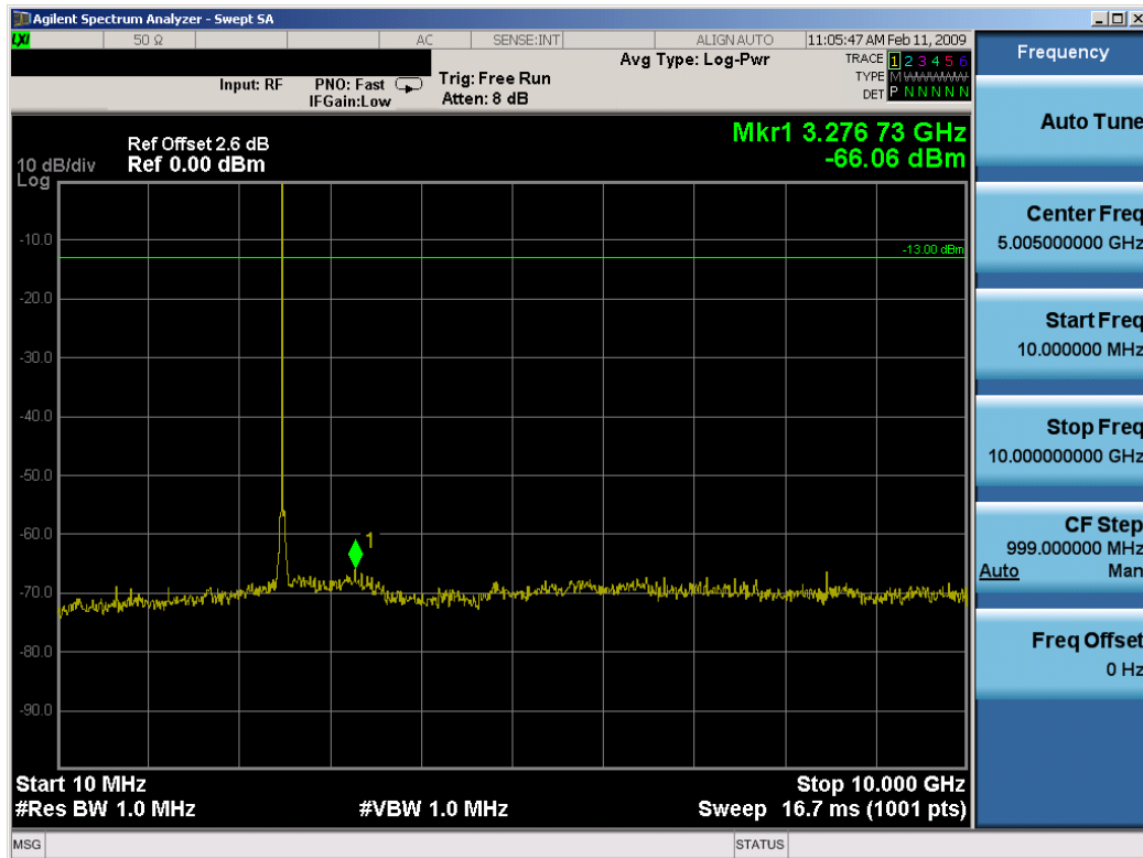
Plot 6-16. Conducted Spurious Plot (Bluetooth – Ch. 78)
