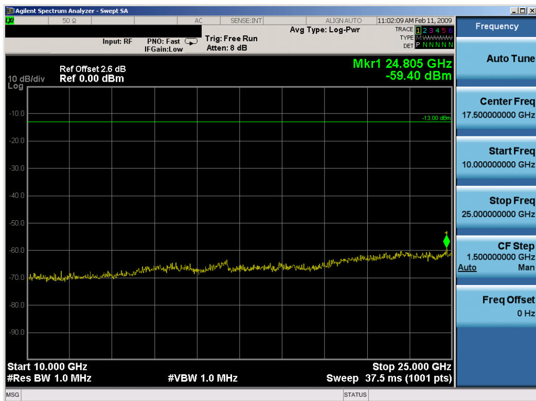
Plot 6-15. Conducted Spurious Plot (Bluetooth – Ch. 39)
