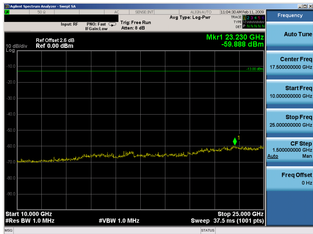
Plot 6-17. Conducted Spurious Plot (Bluetooth – Ch. 78)
