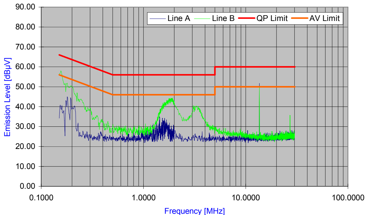
Plot 8-1. Line-Conducted Test Plot
