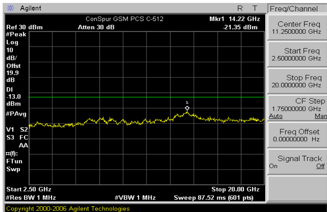
Plot 7-2. Conducted Spurious Plot (PCS GSM Mode – Ch. 512)
