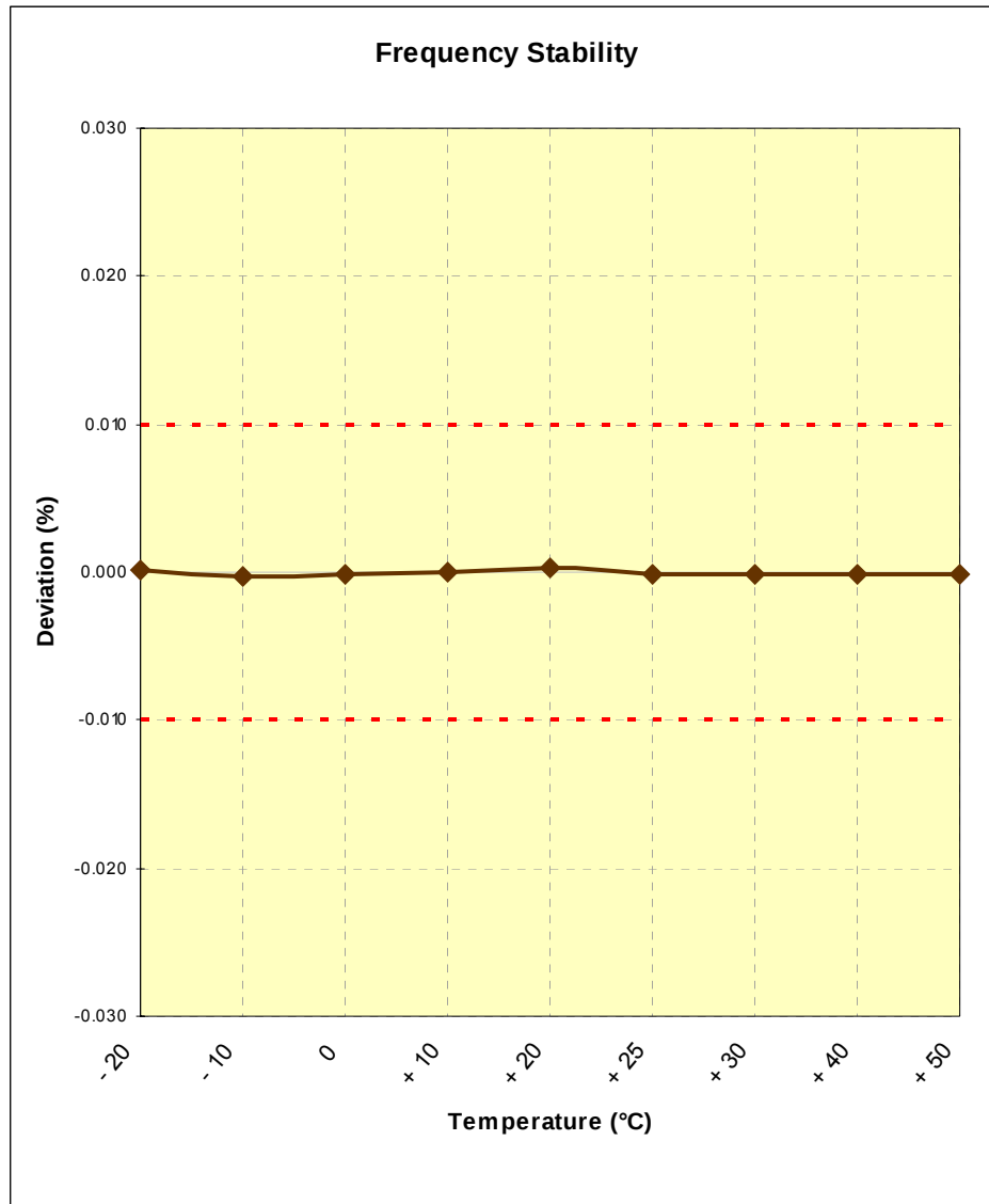
Figure 7-3. Frequency Stability Plot
