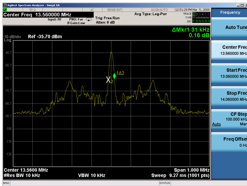
Figure 8-2. Occupied Bandwidth Plot
