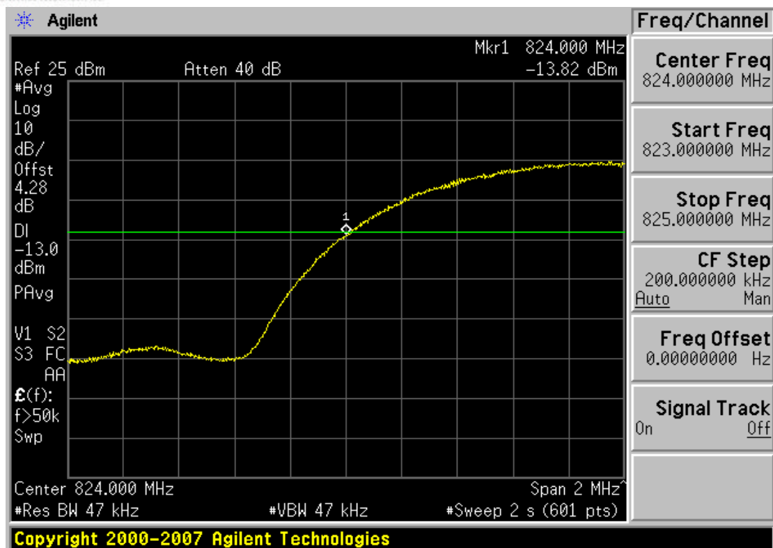
Plot 0-3. Band Edge Plot (Cellular WCDMA Mode – Ch. 4132)
