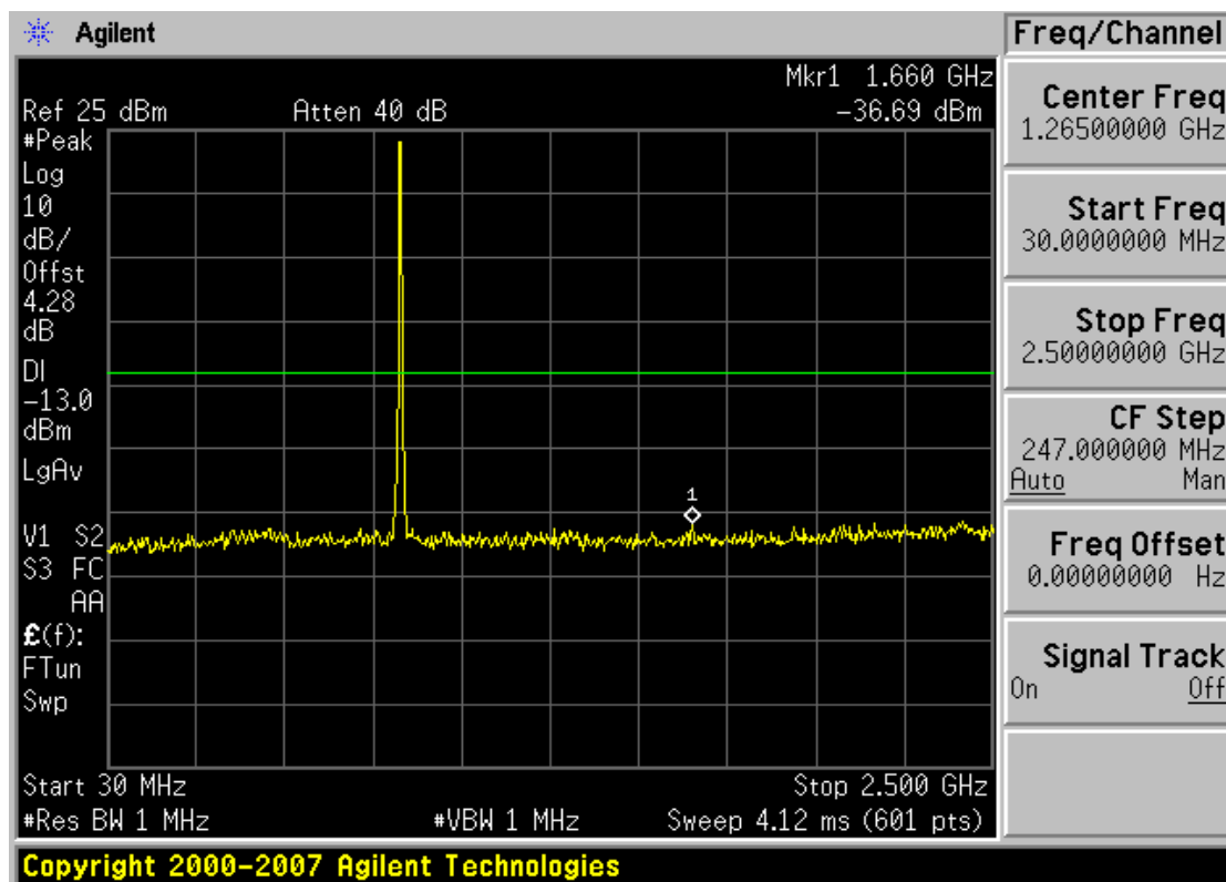
Plot 0-8. Conducted Spurious Plot (Cellular WCDMA Mode – Ch. 4233)
