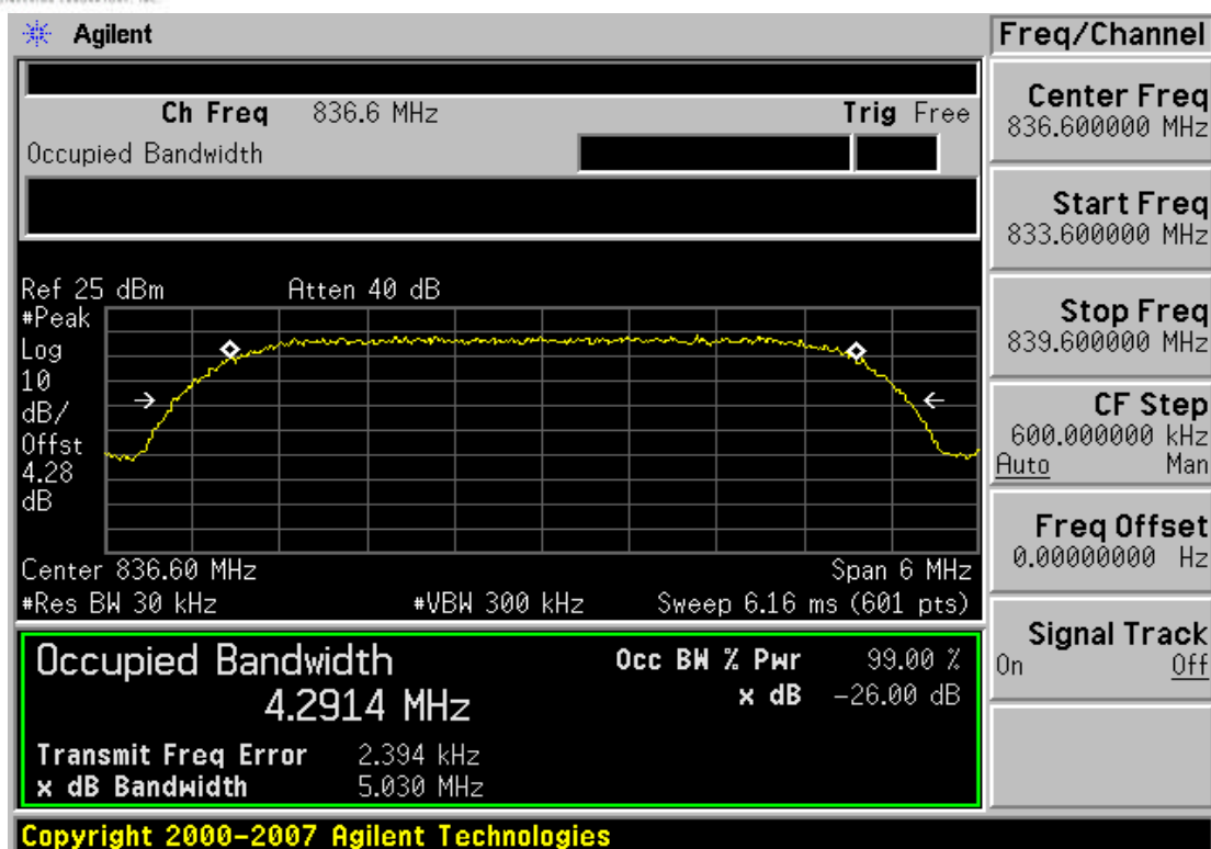
Plot 0-7. Occupied Bandwidth Plot (Cellular WCDMA Mode – Ch. 4183)
