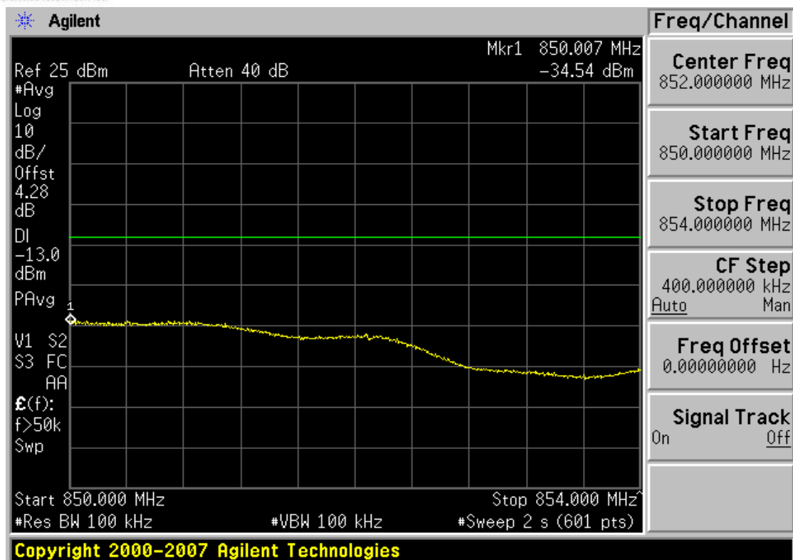
Plot 0-11. 4MHz Span Plot (Cellular WCDMA Mode – Ch. 4233)
