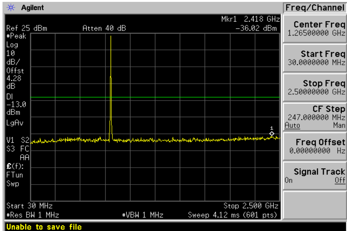
Plot 0-1. Conducted Spurious Plot (Cellular WCDMA Mode – Ch. 4132)
