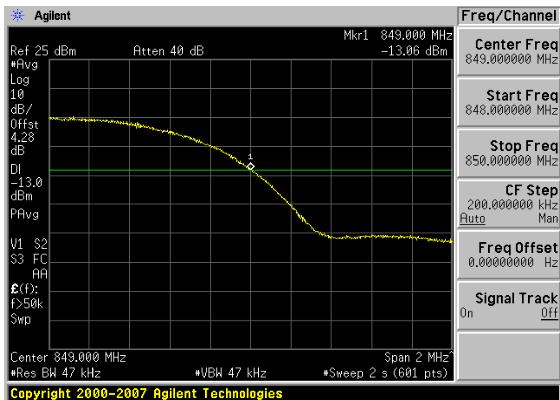
Plot 0-10. Band Edge Plot (Cellular WCDMA Mode – Ch. 4233)
