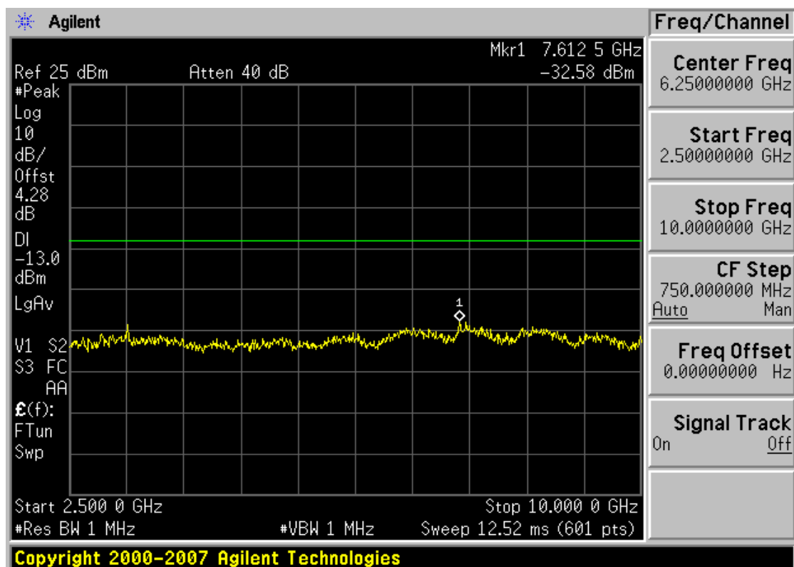
Plot 0-6. Conducted Spurious Plot (Cellular WCDMA Mode – Ch. 4183)
