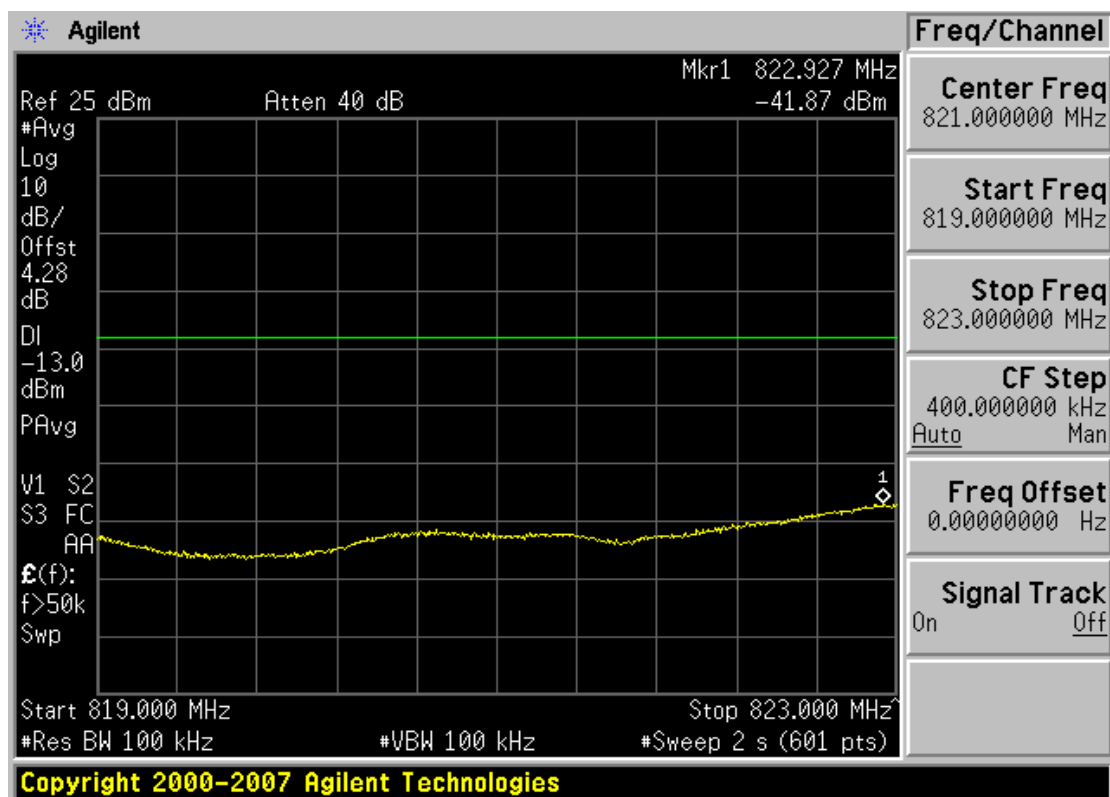
Plot 0-4. 4MHz Span Plot (Cellular WCDMA Mode – Ch. 4132)
