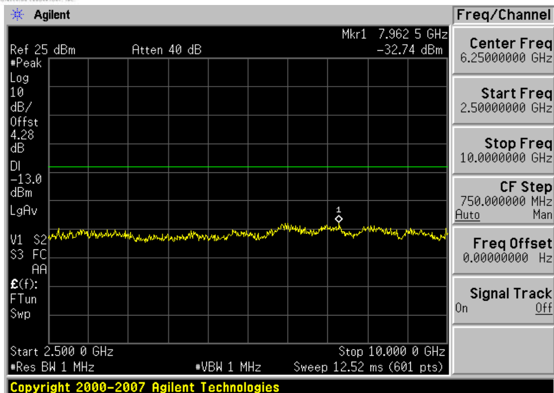
Plot 0-9. Conducted Spurious Plot (Cellular WCDMA Mode – Ch. 4233)
