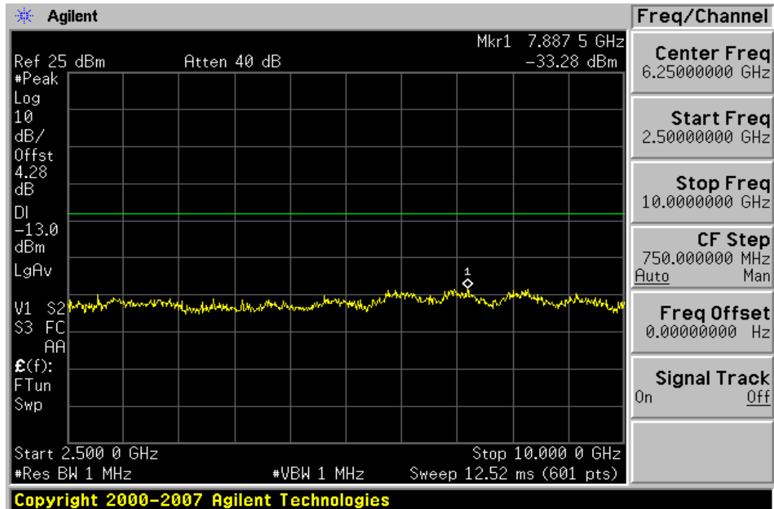
Plot 0-2. Conducted Spurious Plot (Cellular WCDMA Mode – Ch. 4132)
