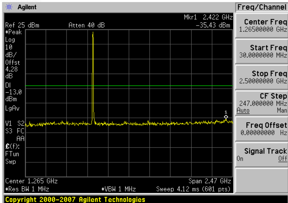
Plot 0-5. Conducted Spurious Plot (Cellular WCDMA Mode – Ch. 4183)
