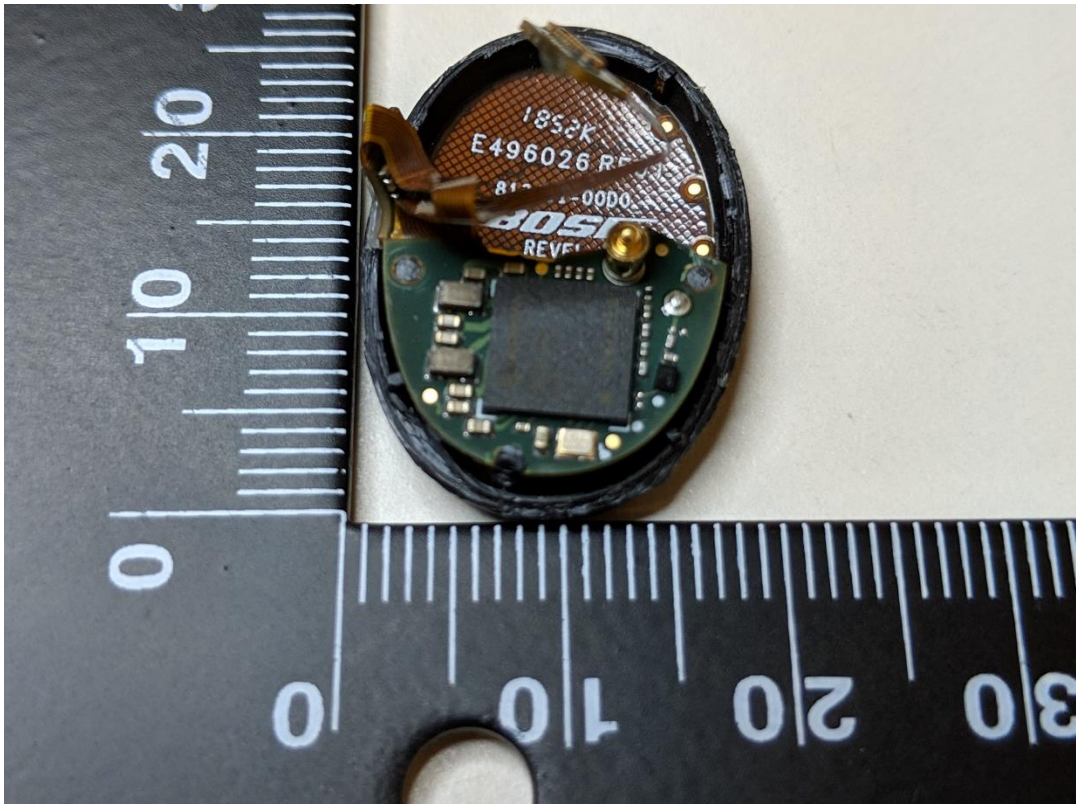
Bose Model BL2R Internal Photos
