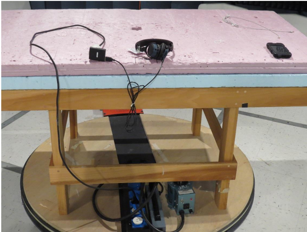
EUT charging mode setup.
