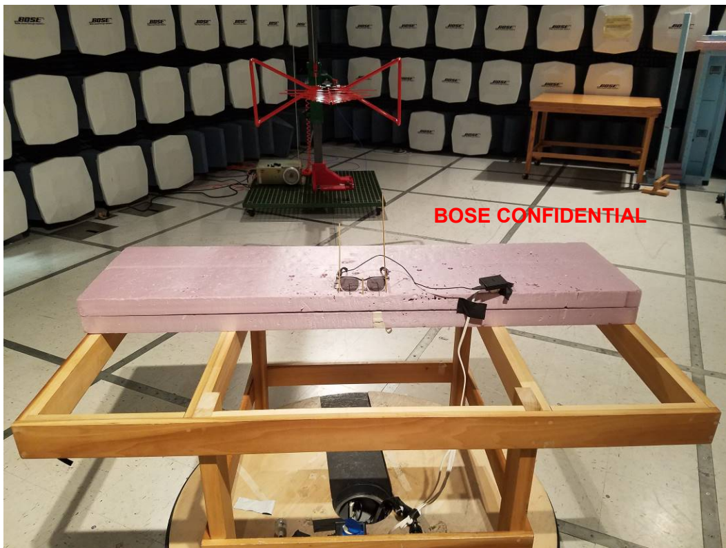
Radiated Emissions 30 MHz to 1 GHz, charging
