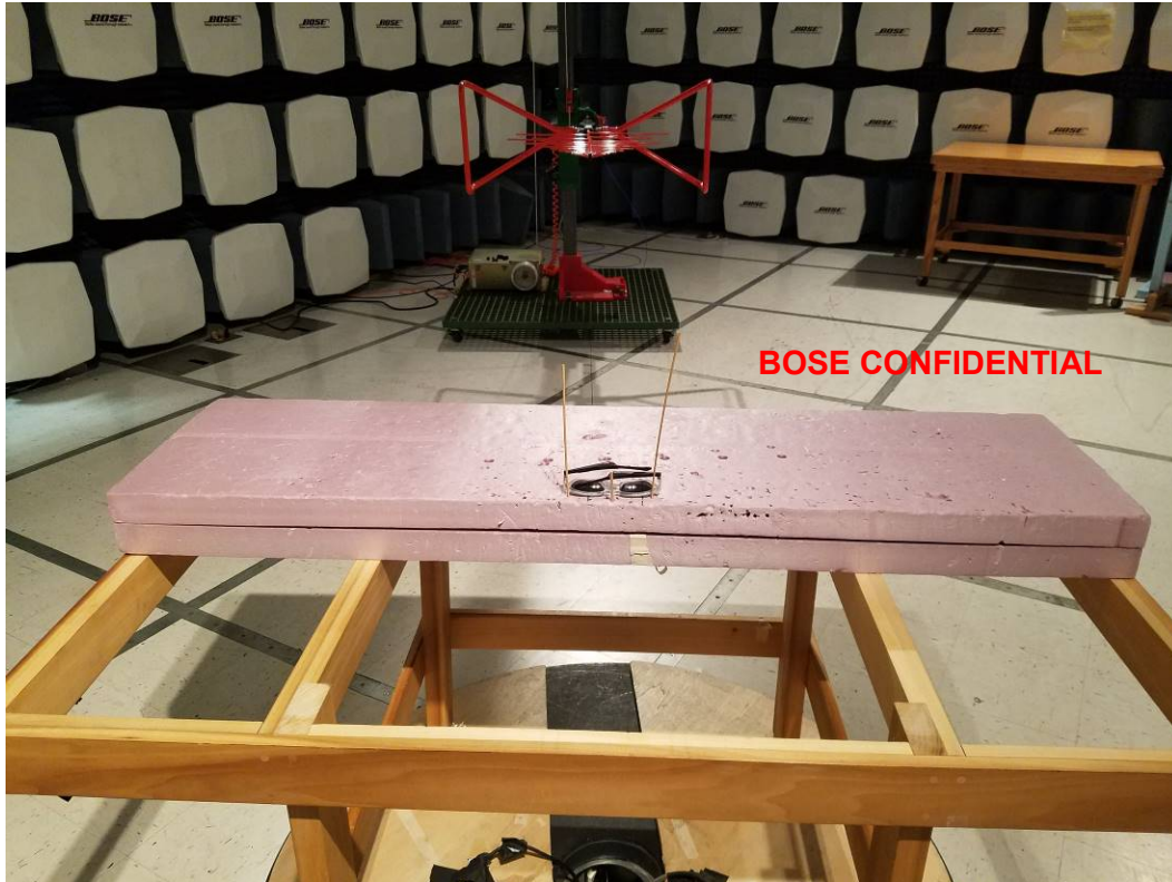
Radiated Emissions 30 MHz to 1 GHz, normal operation
