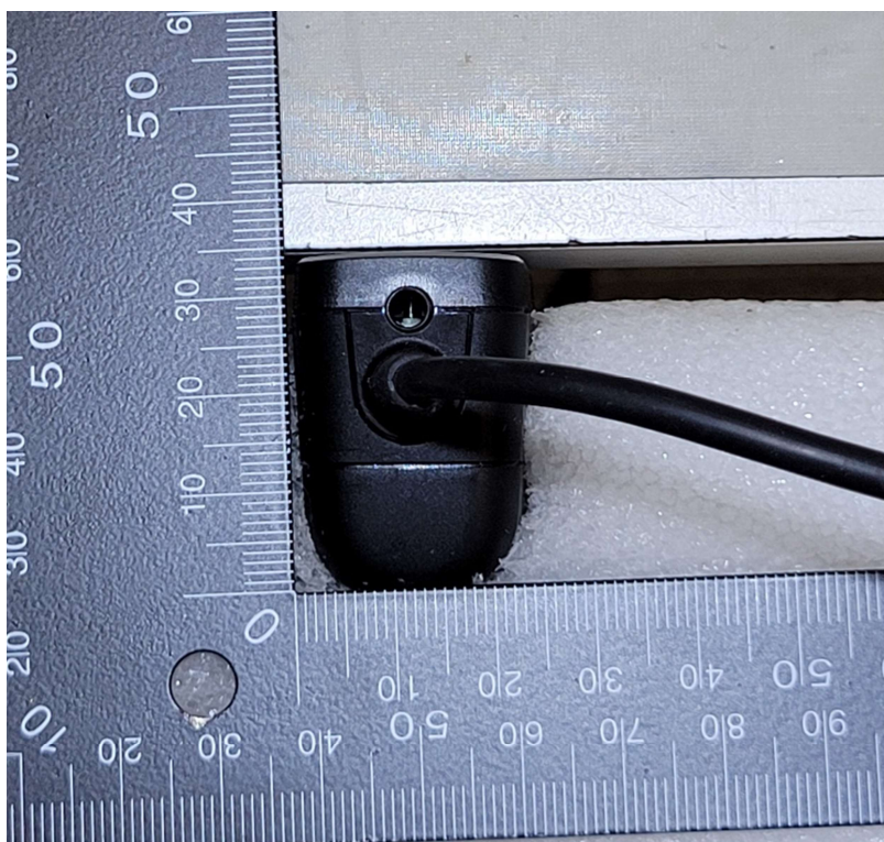
Control module, Aux input end
