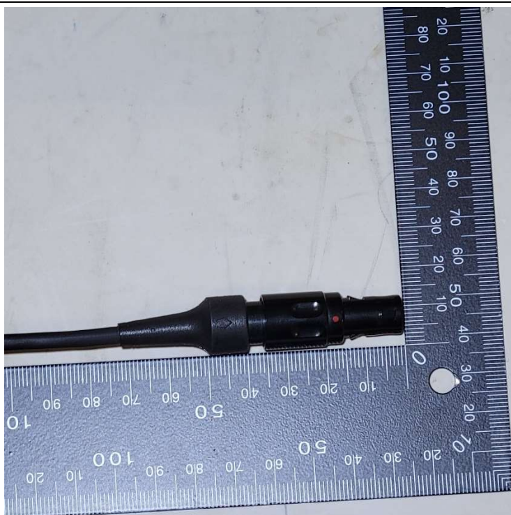
Control module, ICS connector – 6 pin LEMO
