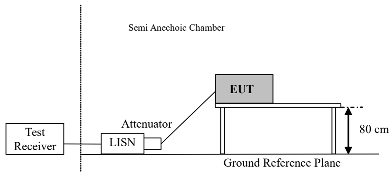
Figure 1: Test Setup
