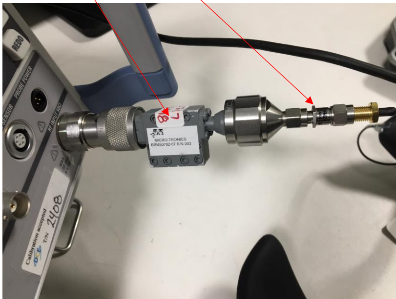
Setup with 2.4 GHz notch filter & 10 dB Pad
