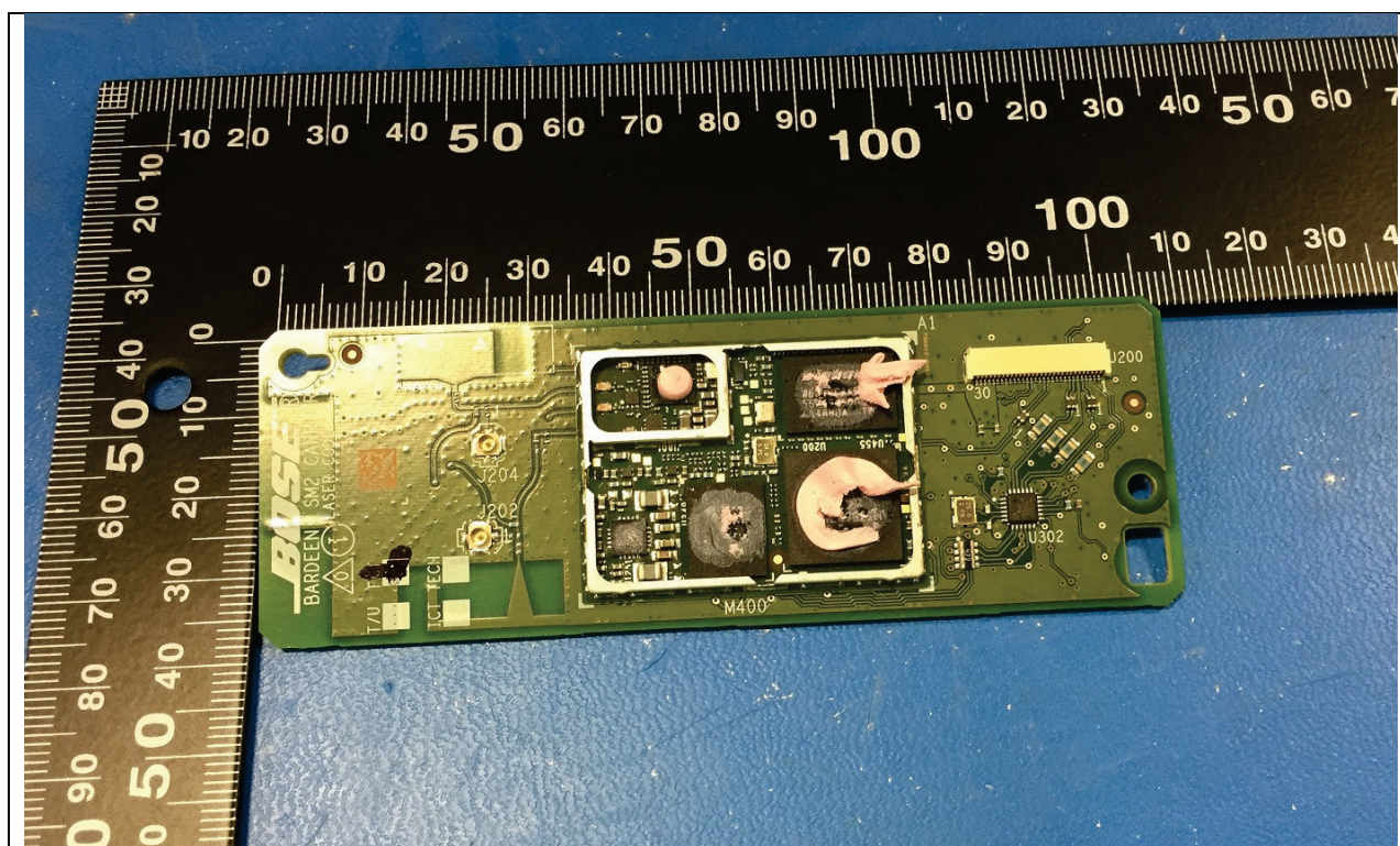
SM2 Board Top (FCC ID: A94416549/IC : 3232A-416549)
