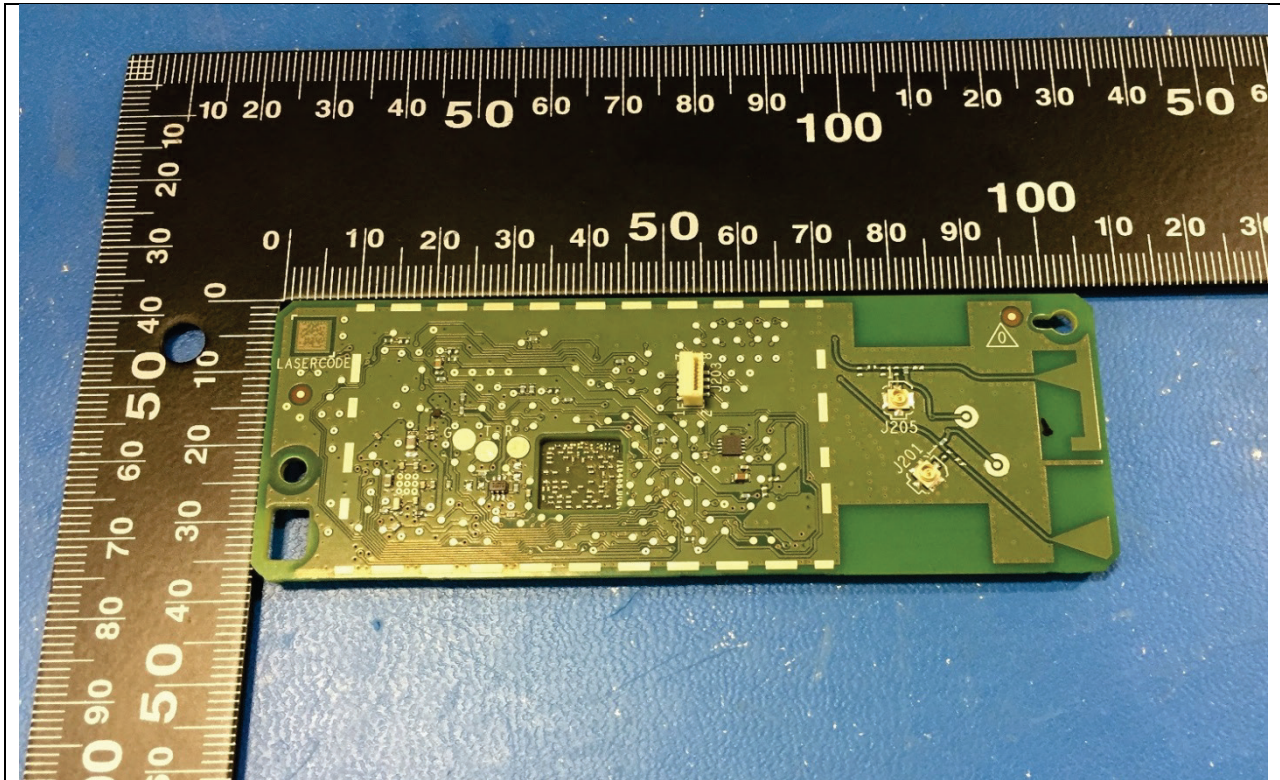
SM2 Board Bottom (FCC ID: A94416549/IC : 3232A-416549)
